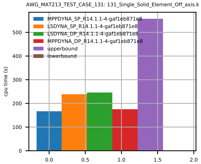
Figure 9: CPU Time.
