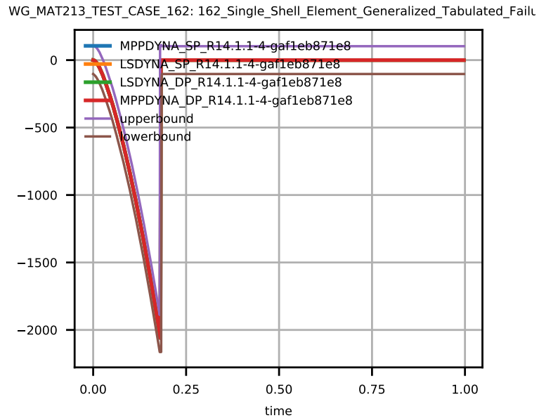
Figure 9: Shell Element Stress \sigma_{xy} at integration point 3.
