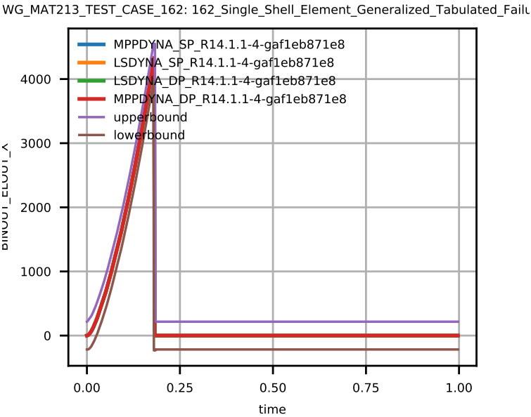
Figure 3: Shell Element Stress xy at integration point 1.
