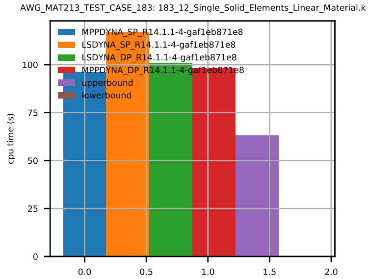
Figure 28: CPU Time.
