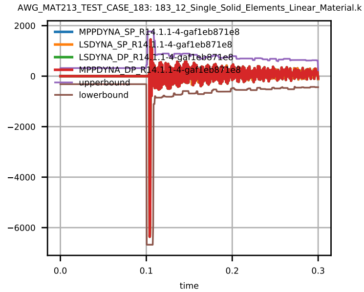
Figure 8: Stress xy of Solid Element 8.
