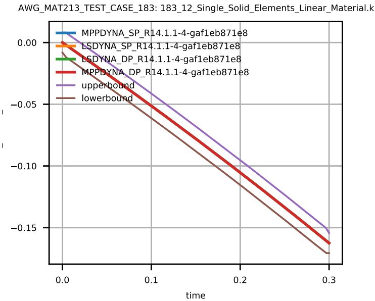
Figure 17: Strain xx of Solid Element 5.
