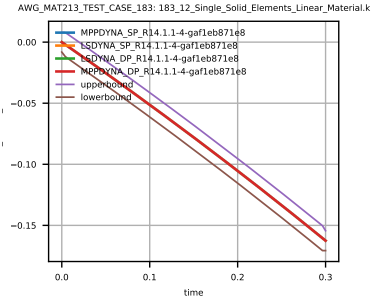
Figure 18: Strain xx of Solid Element 6.
