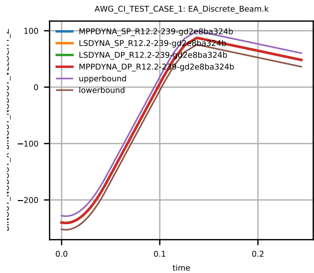
Figure 3: Cross platform results, nodal z velocity node 2
