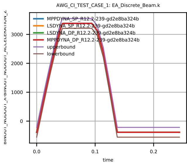
Figure 4: Cross platform results, nodal z acceleration node 2
