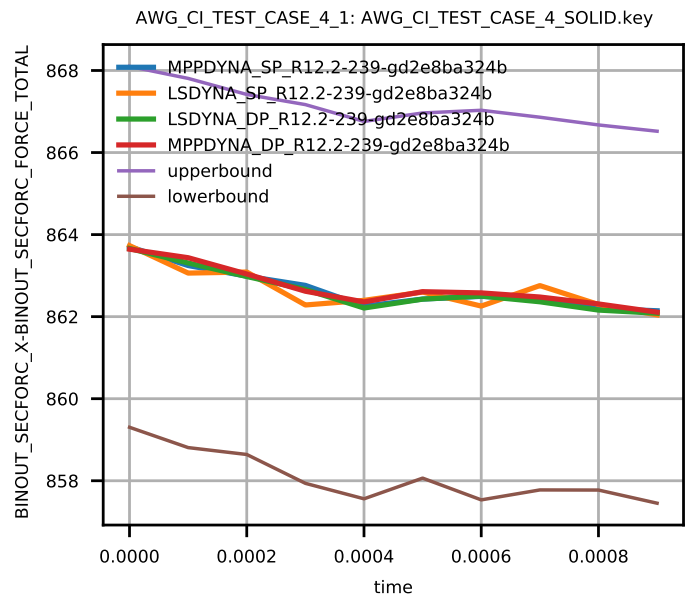
Figure 2: Resultant Force, Bolt Cross-Section plane.
