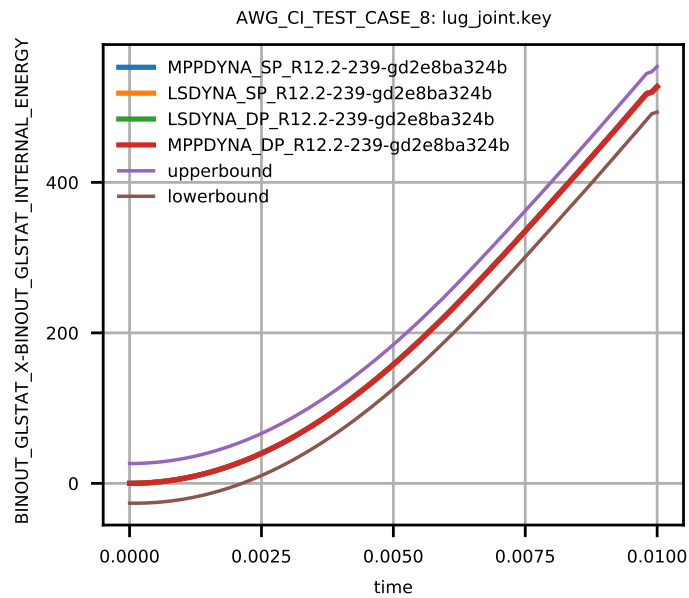
Figure 4: Internal Energy.
