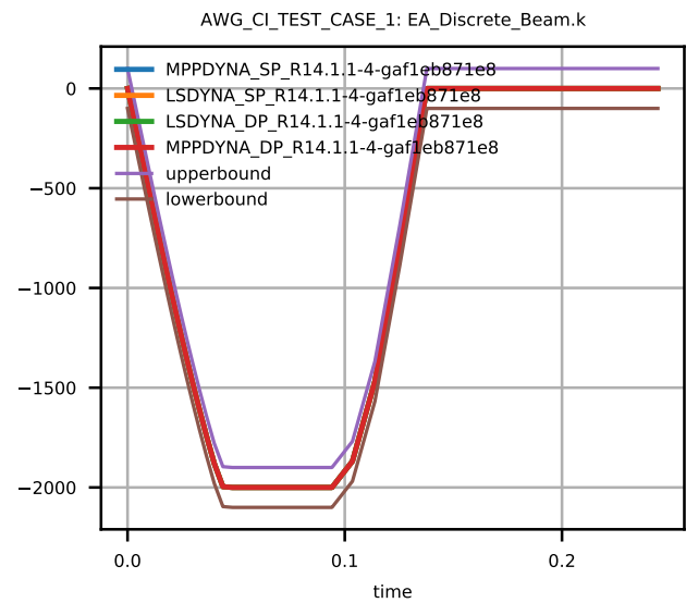
Figure 5: Cross platform results, axial force resultant beam 1
