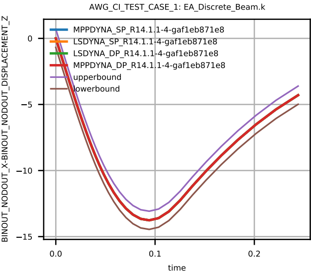
Figure 2: Cross platform results, nodal z displacement node 2
