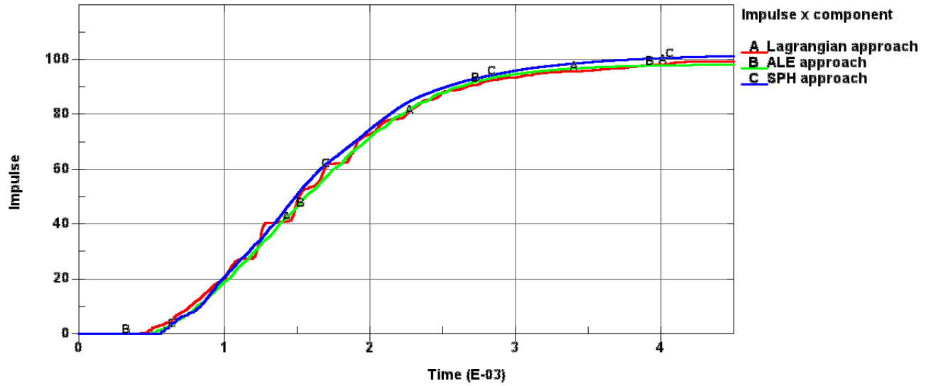
Figure 11: Platform averaged impulse for the different modelling approaches
