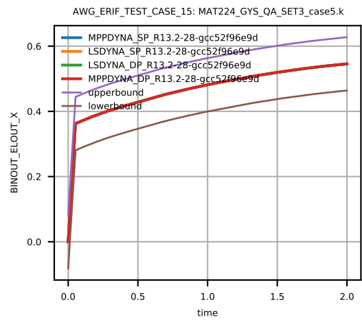
Figure 110: Cross platform results, Von Mises Stress, element ID 2, sub test case ID 7
