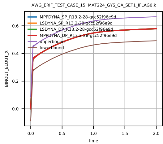
Figure 4: Cross platform results, z-component Stress, element ID 1, sub test case ID 1
