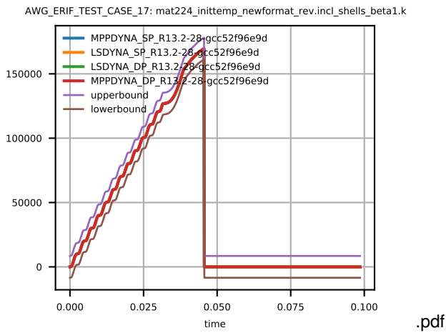
Figure 3: Cross platform results, Von Mises Stress, element ID 4, sub test case ID 2
