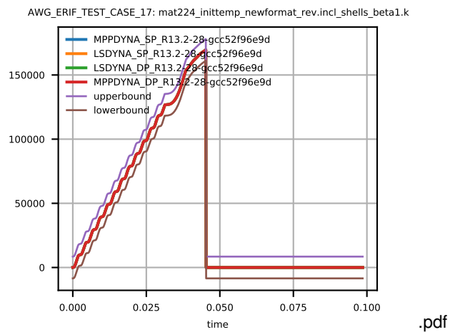
Figure 9: Cross platform results, Von Mises Stress, element ID 14, sub test case ID 2
