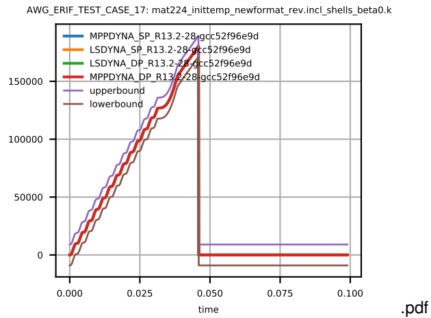
Figure 8: Cross platform results, Von Mises Stress, element ID 14, sub test case ID 1
