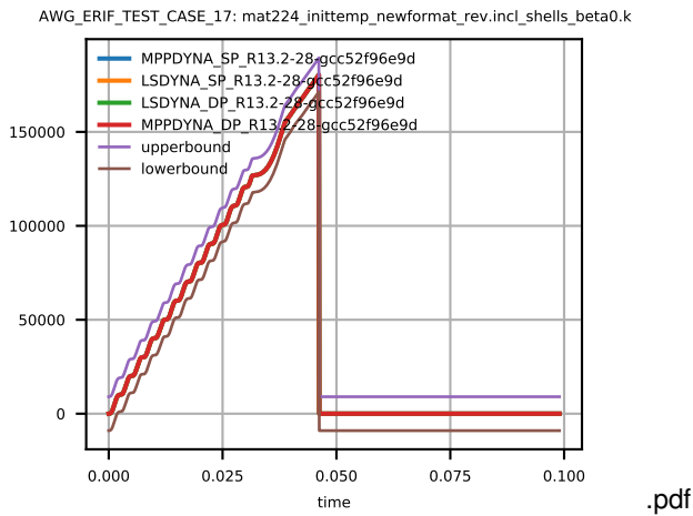
Figure 2: Cross platform results, Von Mises Stress, element ID 4, sub test case ID 1
