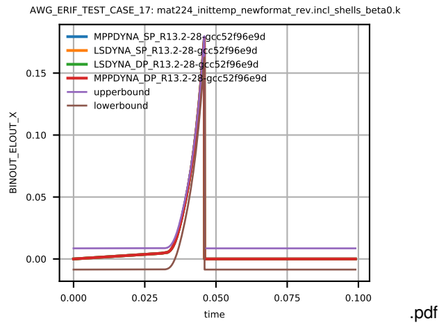
Figure 10: Cross platform results, Effective Plastic Strain, element ID 14, sub test case ID 1
