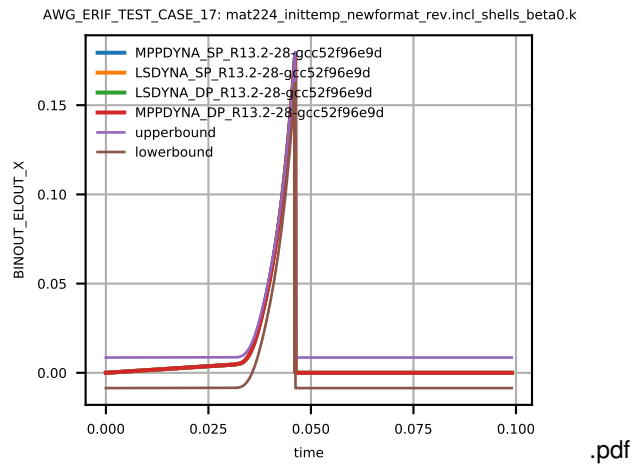
Figure 4: Cross platform results, Effective Plastic Strain, element ID 4, sub test case ID 1
