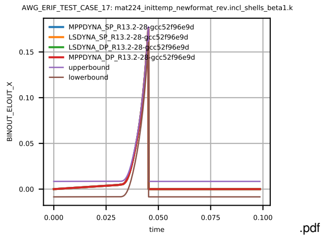
Figure 11: Cross platform results, Effective Plastic Strain, element ID 14, sub test case ID 2
