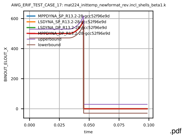
Figure 13: Cross platform results, History Variable 10 (temperature), element ID 14, sub test case ID 2
