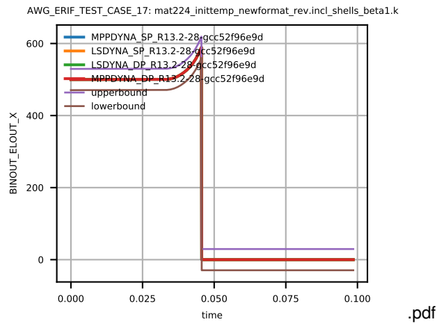
Figure 7: Cross platform results, History Variable 14 (temperature), element ID 4, sub test case ID 2
