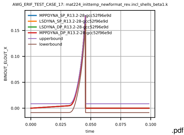
Figure 5: Cross platform results, Effective Plastic Strain, element ID 4, sub test case ID 2
