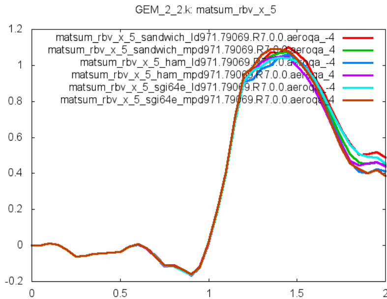
Figure 6: Cross platform results, rigid body velocity x component Part 5 (released fan blade), sub test case ID 1
