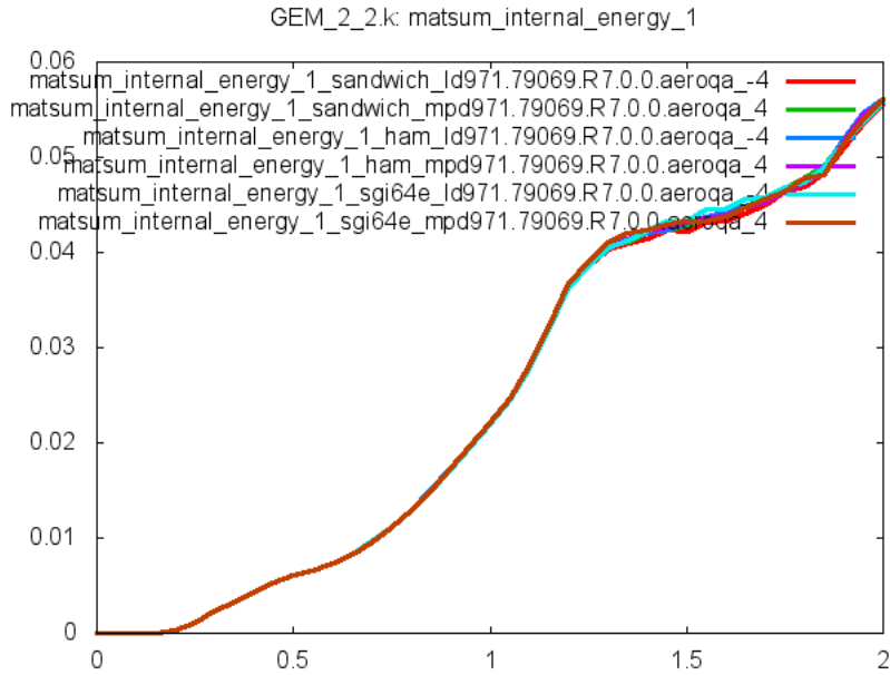
Figure 9: Cross platform results, internal energy Part 1 (casing), sub test case ID 1
