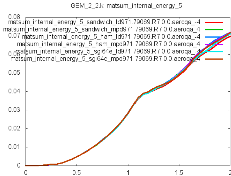
Figure 4: Cross platform results, internal energy Part 5 (released fan blade), sub test case ID 1
