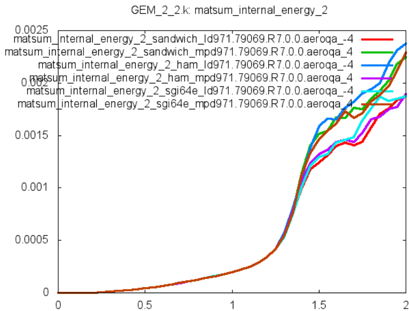
Figure 10: Cross platform results, internal energy Part 2 (fabric), sub test case ID 1
