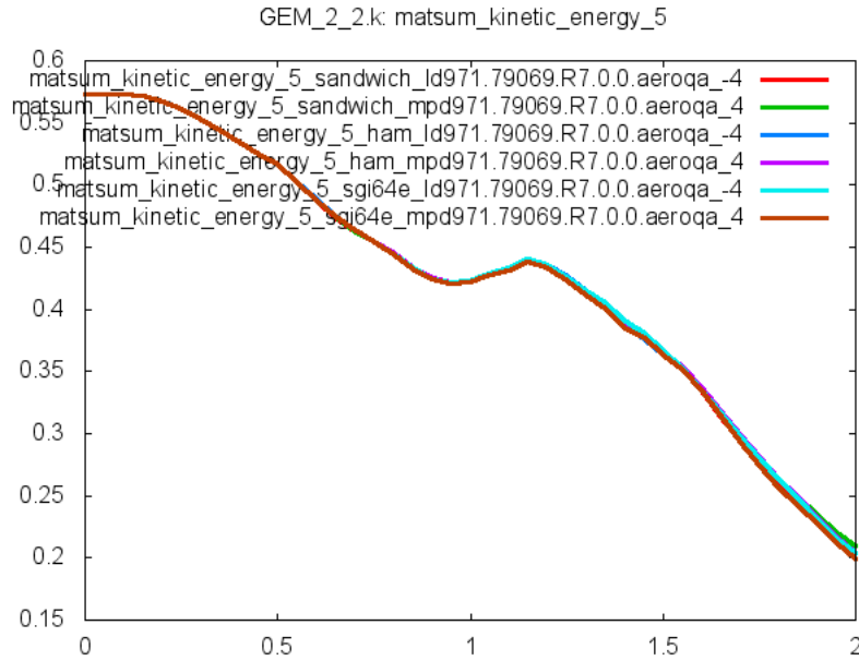
Figure 5: Cross platform results, kinetic energy Part 5 (released fan blade), sub test case ID 1
