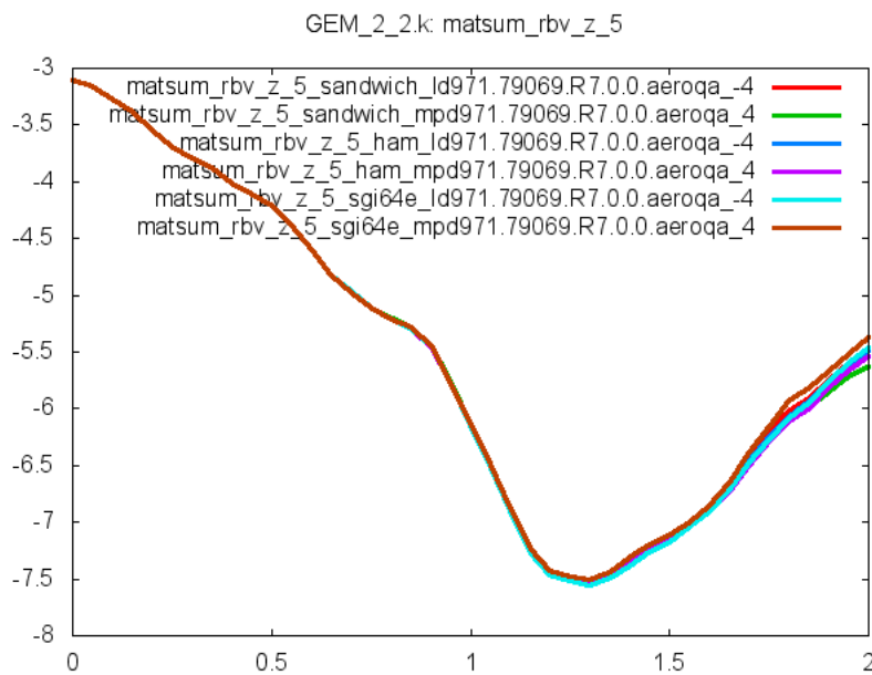
Figure 8: Cross platform results, rigid body velocity z component Part 5 (released fan blade), sub test case ID 1
