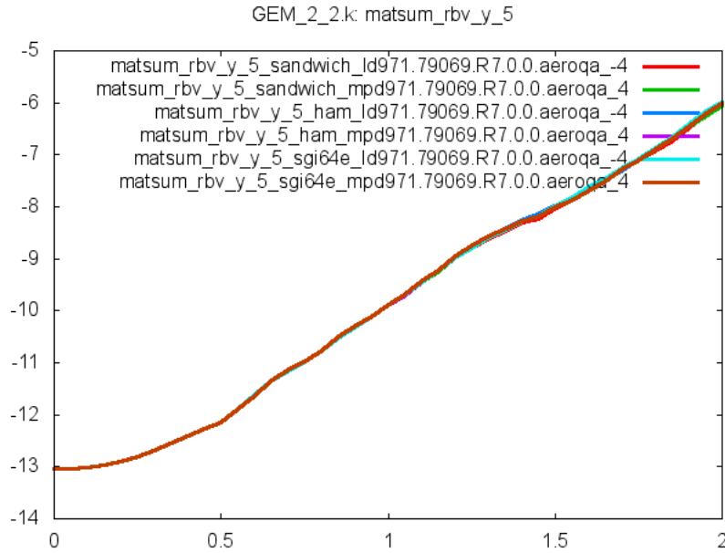
Figure 7: Cross platform results, rigid body velocity y component Part 5 (released fan blade), sub test case ID 1
