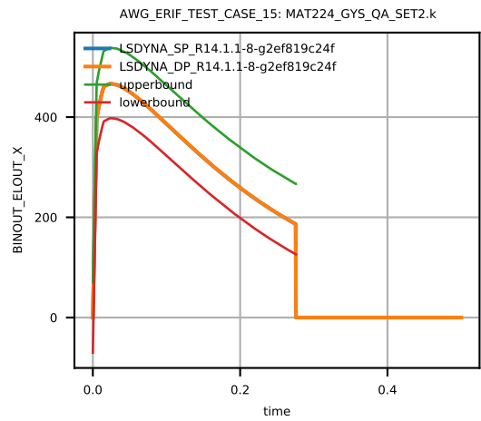
Figure 45: Cross platform results, z-component Stress, element ID 10, sub test case ID 3
