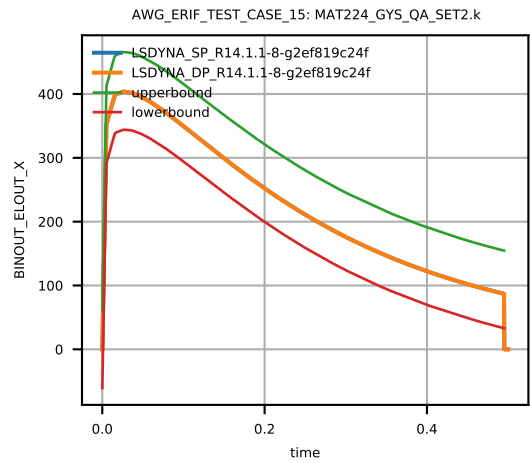
Figure 44: Cross platform results, z-component Stress, element ID 9, sub test case ID 3
