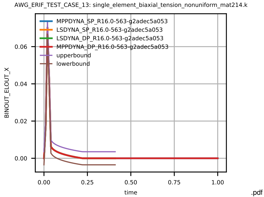
Figure 11: Cross platform results, stress in x-direction, integration point 1, sub test case ID 7
