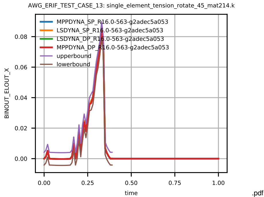
Figure 7: Cross platform results, stress in x-direction, integration point 1, sub test case ID 5
