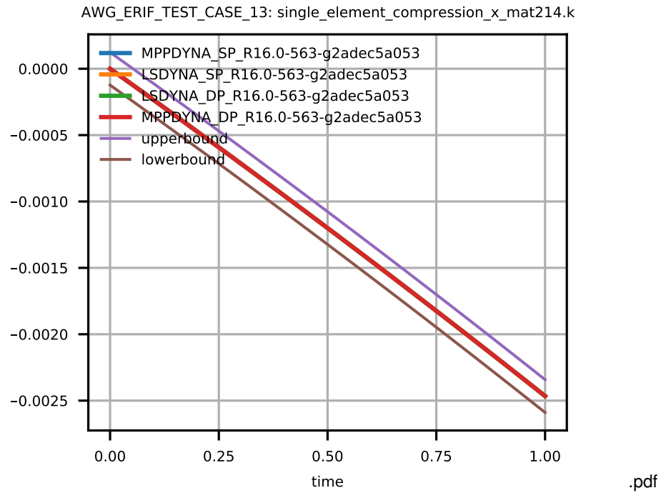
Figure 5: Cross platform results, stress in x-direction, integration point 1, sub test case ID 3
