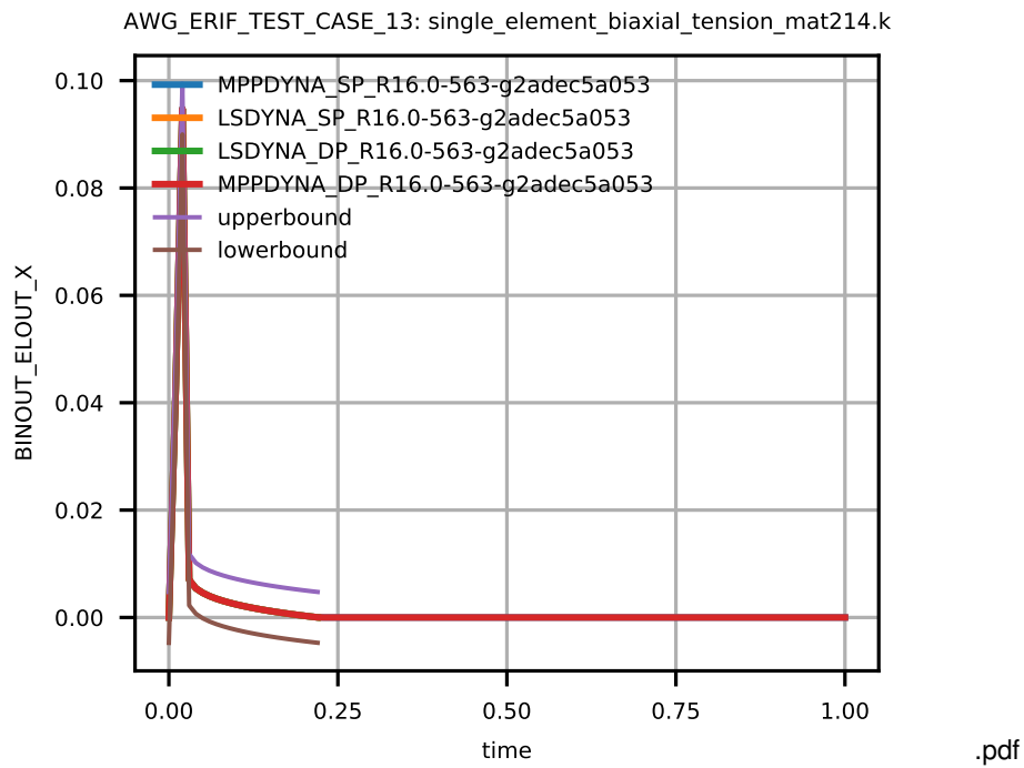
Figure 10: Cross platform results, stress in y-direction, integration point 1, sub test case ID 6
