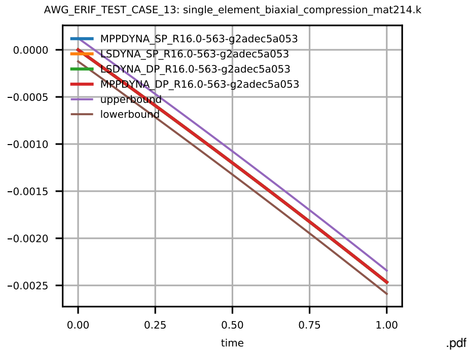
Figure 13: Cross platform results, stress in x-direction, integration point 1, sub test case ID 8
