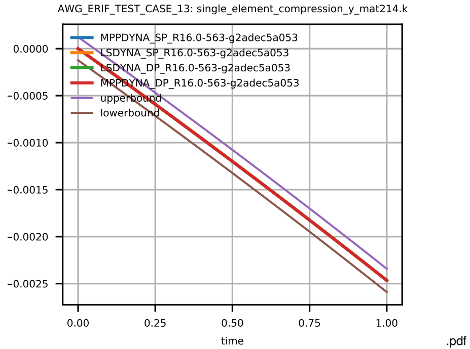
Figure 6: Cross platform results, stress in y-direction, integration point 1, sub test case ID 4
