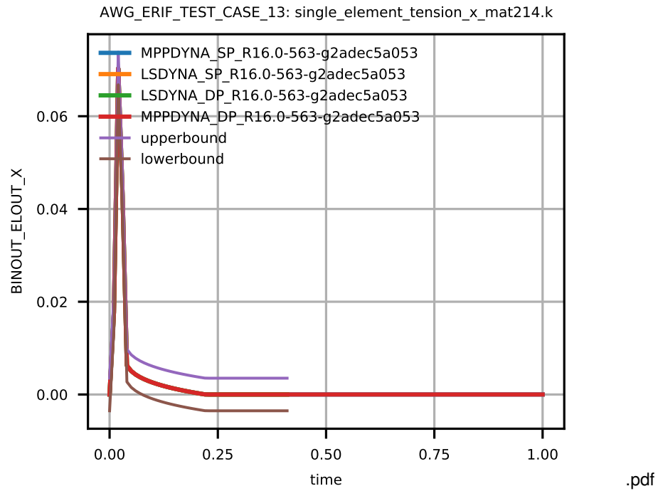
Figure 3: Cross platform results, stress in x-direction, integration point 1, sub test case ID 1
