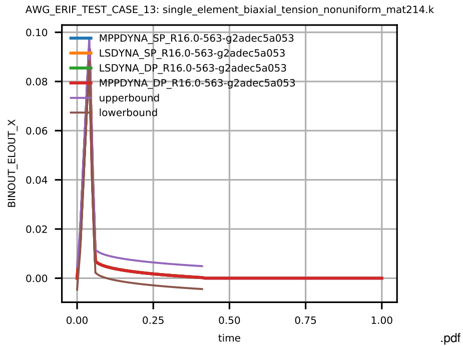
Figure 12: Cross platform results, stress in y-direction, integration point 1, sub test case ID 7
