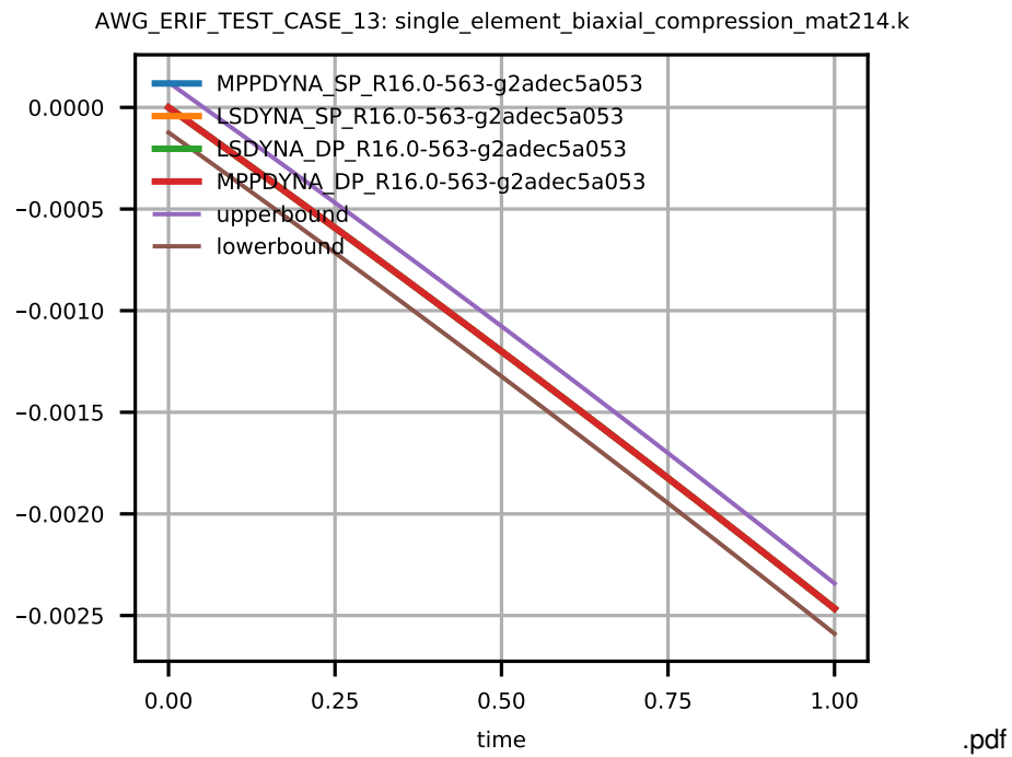
Figure 14: Cross platform results, stress in y-direction, integration point 1, sub test case ID 8
