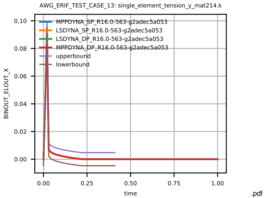
Figure 4: Cross platform results, stress in y-direction, integration point 1, sub test case ID 2
