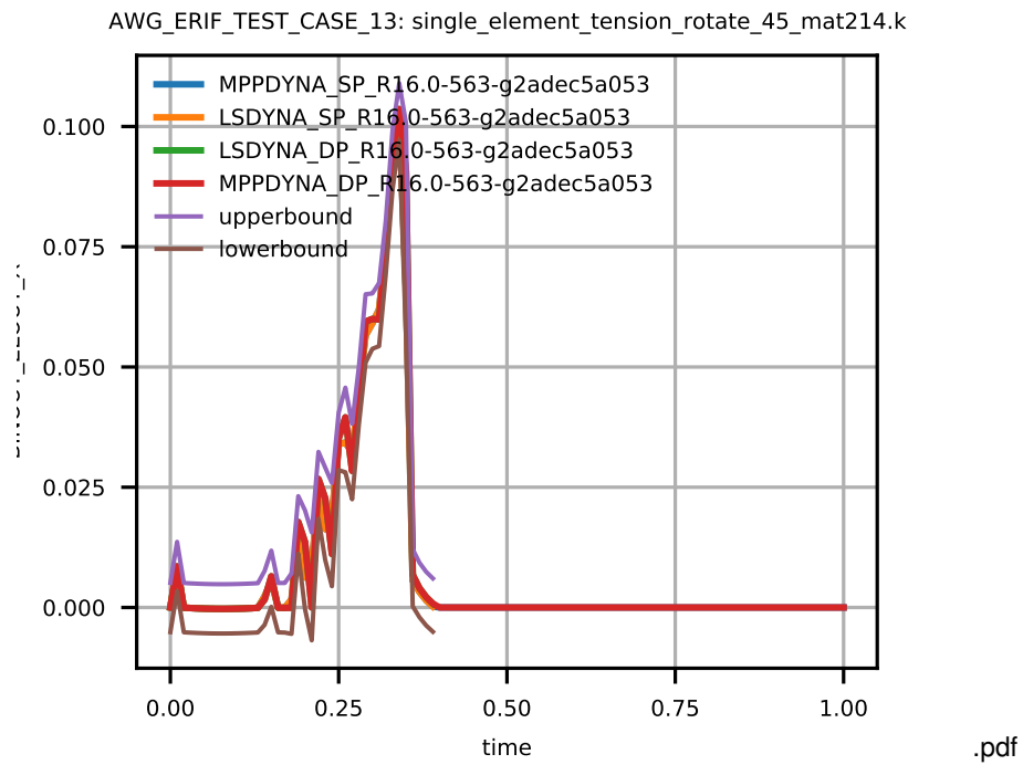
Figure 8: Cross platform results, stress in y-direction, integration point 1, sub test case ID 5
