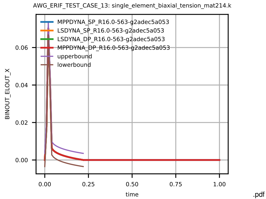
Figure 9: Cross platform results, stress in x-direction, integration point 1, sub test case ID 6
