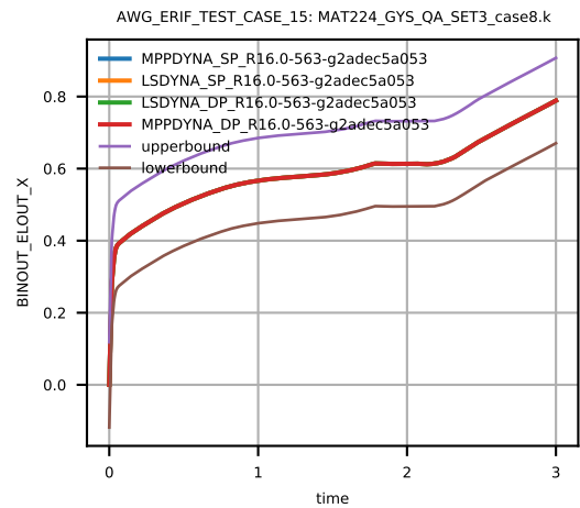
Figure 147: Cross platform results, Von Mises Stress, element ID 3, sub test case ID 10
