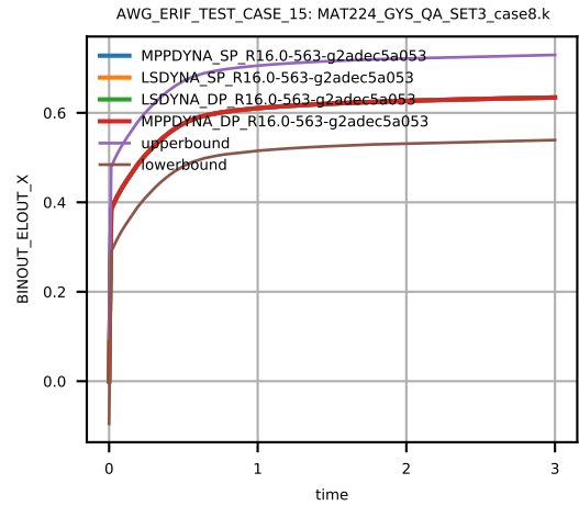
Figure 146: Cross platform results, Von Mises Stress, element ID 2, sub test case ID 10
