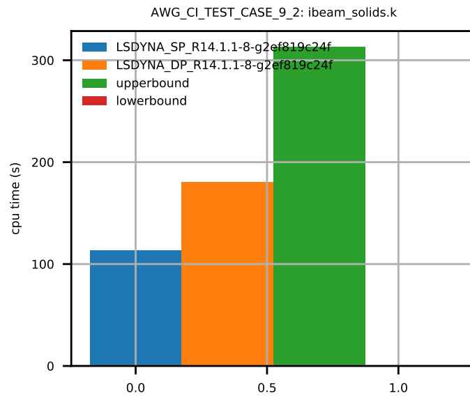
Figure 9: CPU Time Comparison.
