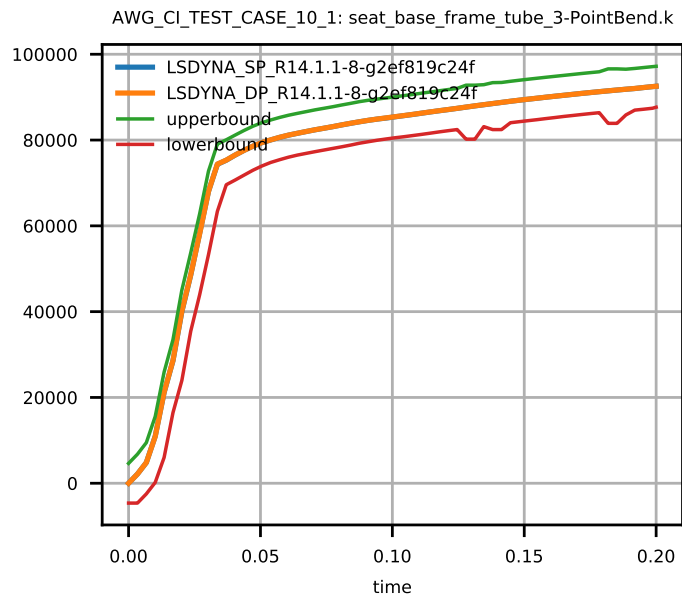
Figure 4: Von Mises Stress of Element 981.
