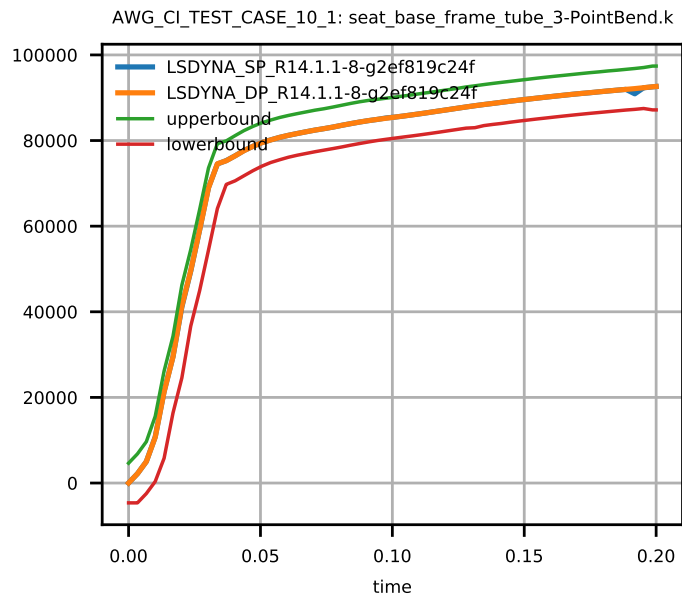
Figure 5: Von Mises Stress of Element 993.
