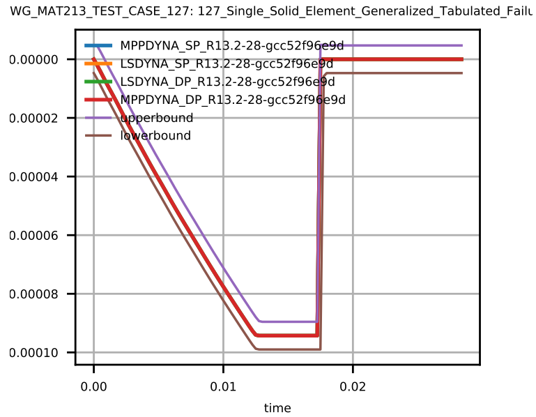
Figure 8: Solid Element Strain yy.
