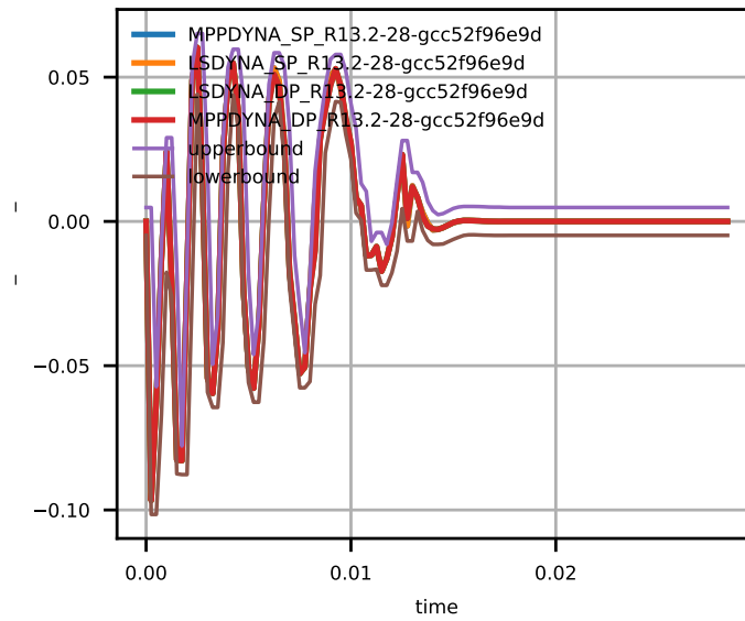
Figure 4: Solid Element Stress xy.
