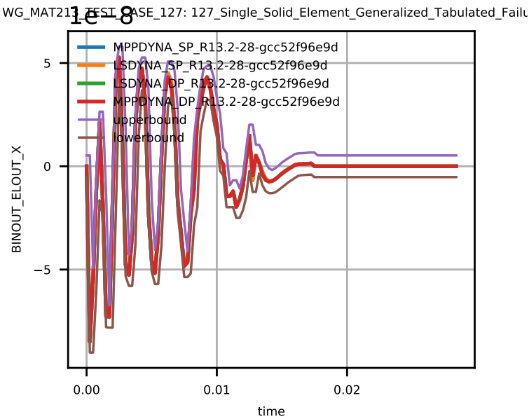
Figure 10: Solid Element Strain xy.
