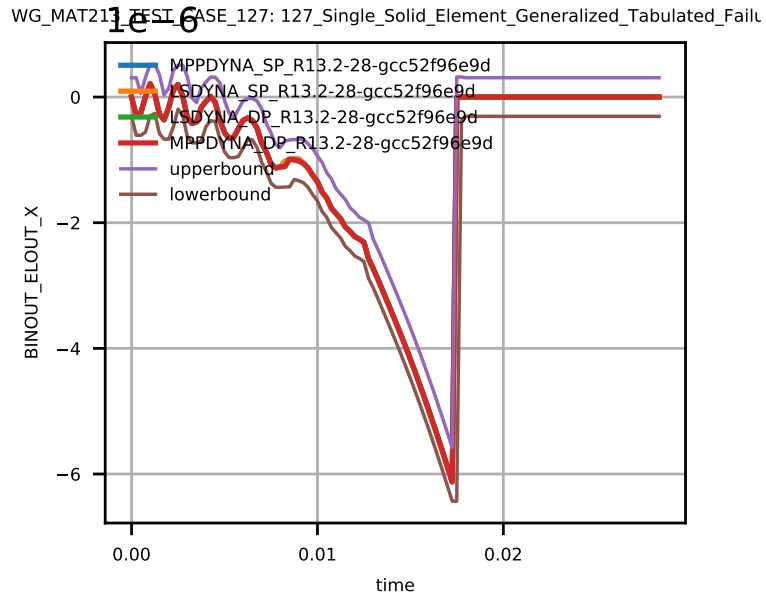
Figure 11: Solid Element Strain yz.
