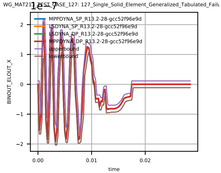
Figure 12: Solid Element Strain zx.
