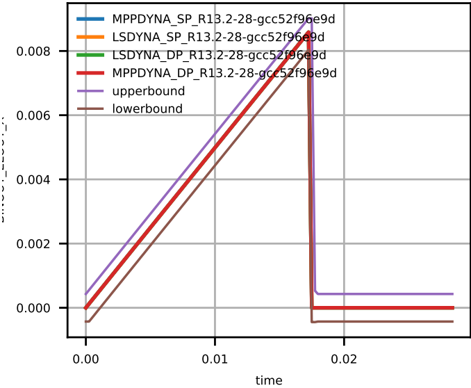
Figure 7: Solid Element Strain xx.
