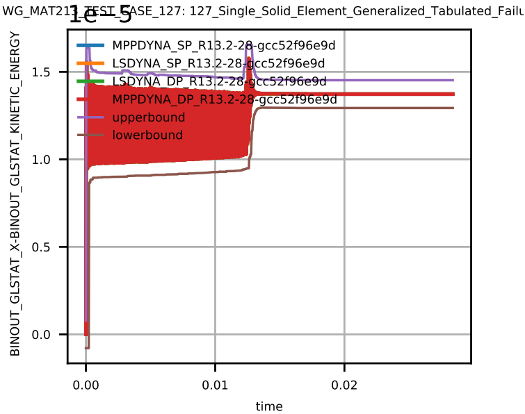
Figure 15: Global Kinetic Energy.
