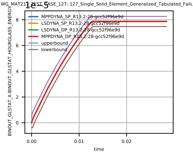
Figure 16: Global Hourglass Energy.
