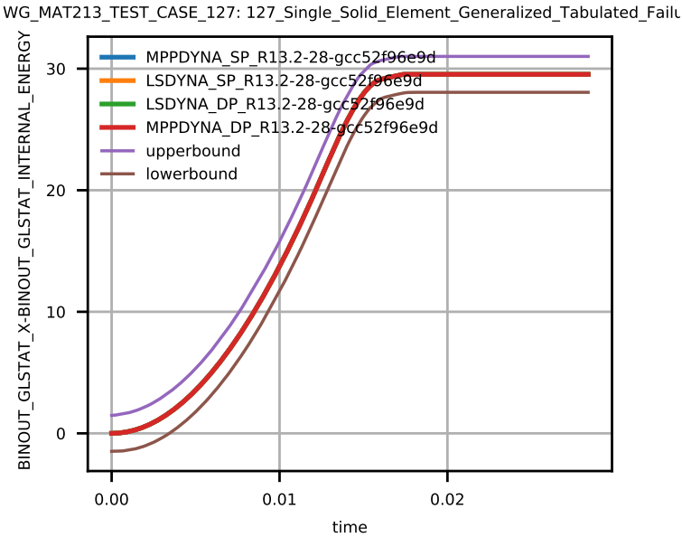
Figure 14: Global Internal Energy.
