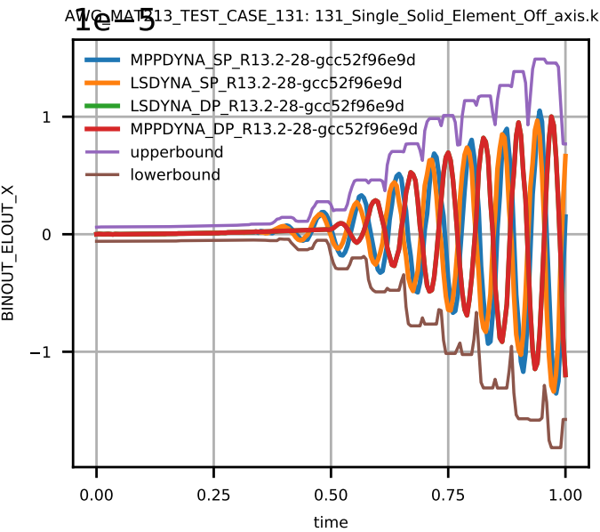
Figure 6: Solid Element Strain zx.
