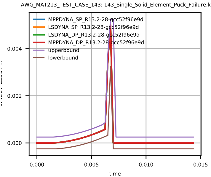
Figure 13: Solid Element Strain zx.
