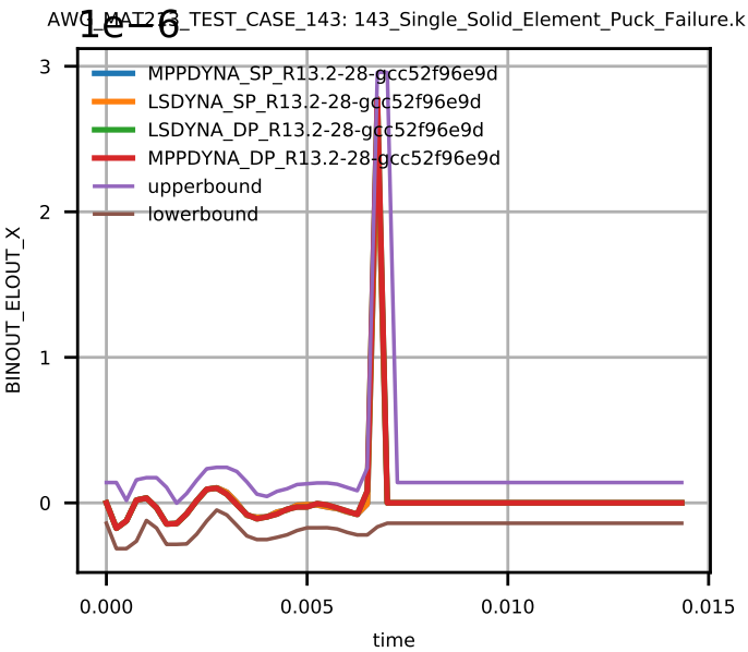
Figure 10: Solid Element Strain xy.
