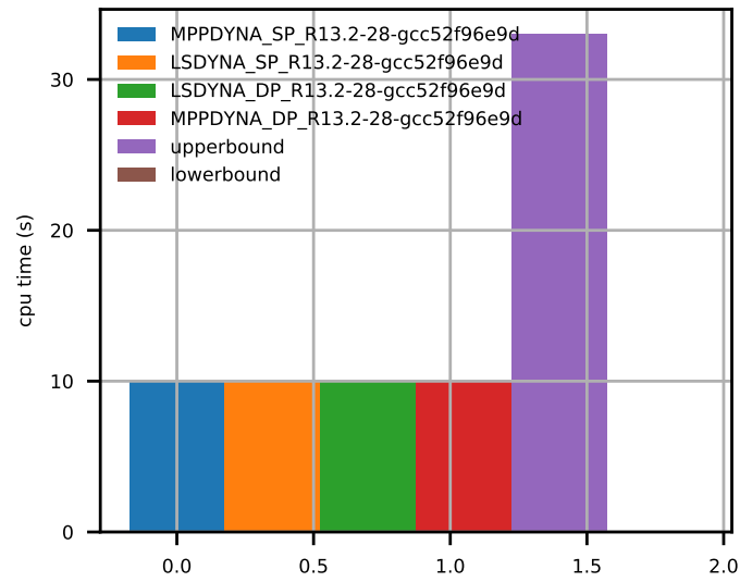
Figure 19: CPU Time.
