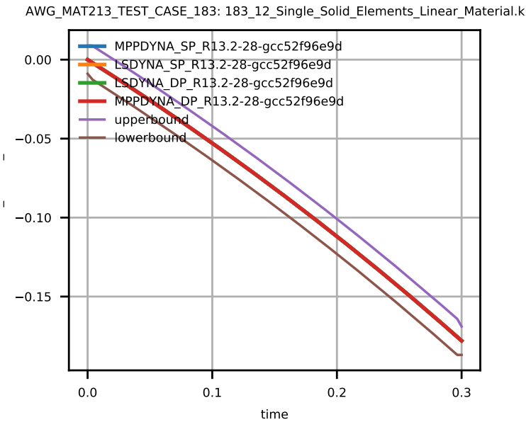
Figure 24: Strain xx of Solid Element 12.
