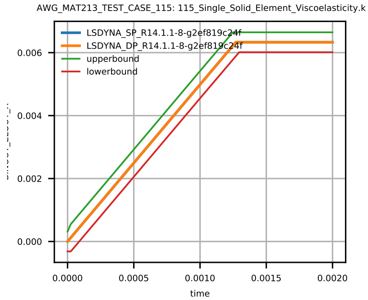
Figure 7: Solid Element Strain xx.
