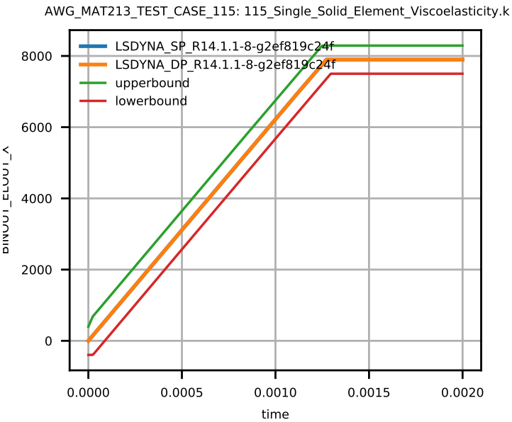
Figure 1: Solid Element Stress xx.
