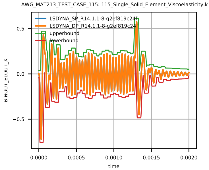
Figure 6: Solid Element Stress zx.
