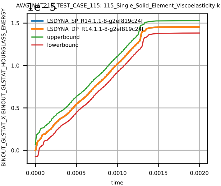
Figure 10: Global Hourglass Energy.
