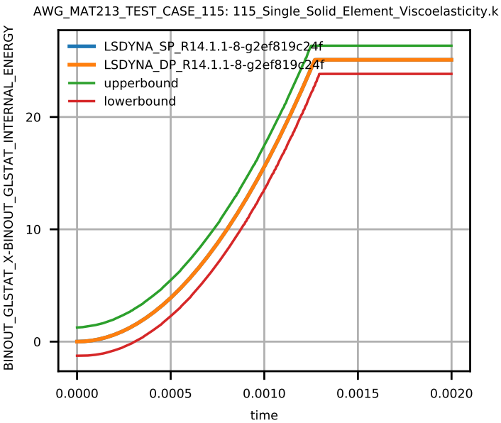
Figure 8: Global Internal Energy.
