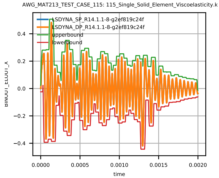
Figure 4: Solid Element Stress xy.
