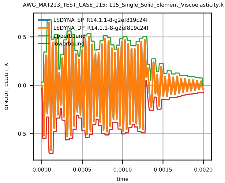
Figure 5: Solid Element Stress yz.
