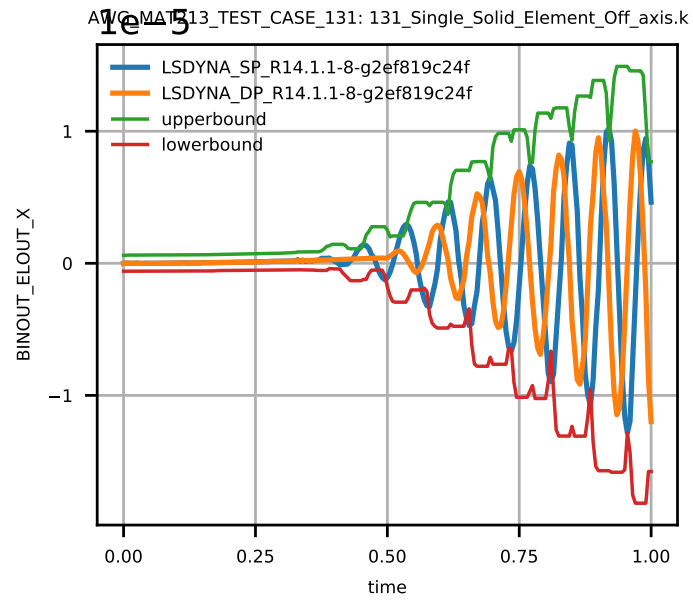
Figure 6: Solid Element Strain zx.
