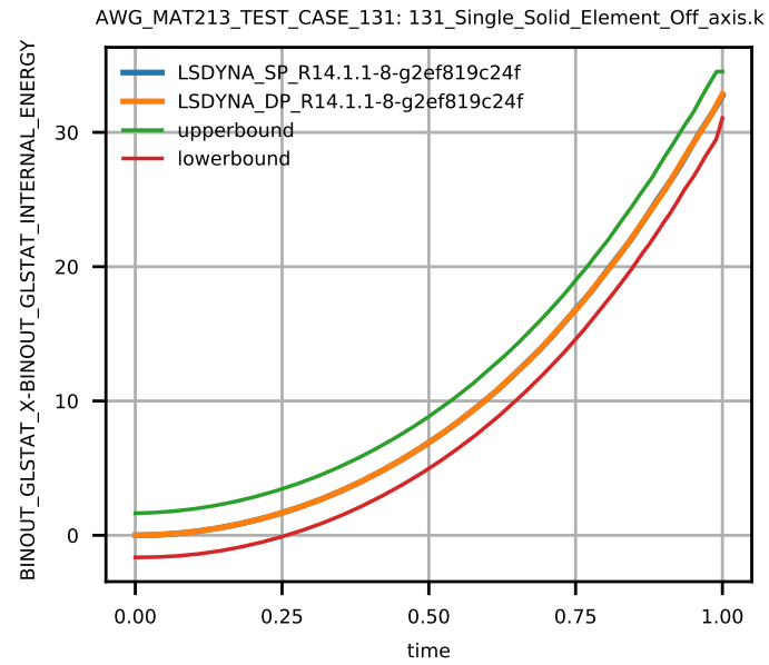
Figure 7: Global Internal Energy.
