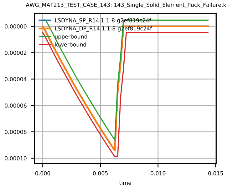
Figure 8: Solid Element Strain \epsilon_{yy} .
