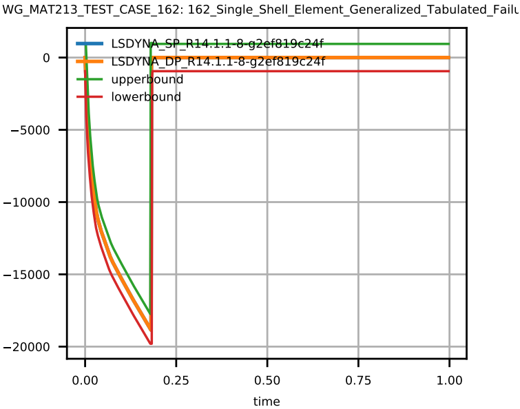
Figure 7: Shell Element Stress \sigma_{xx} at integration point 3.
