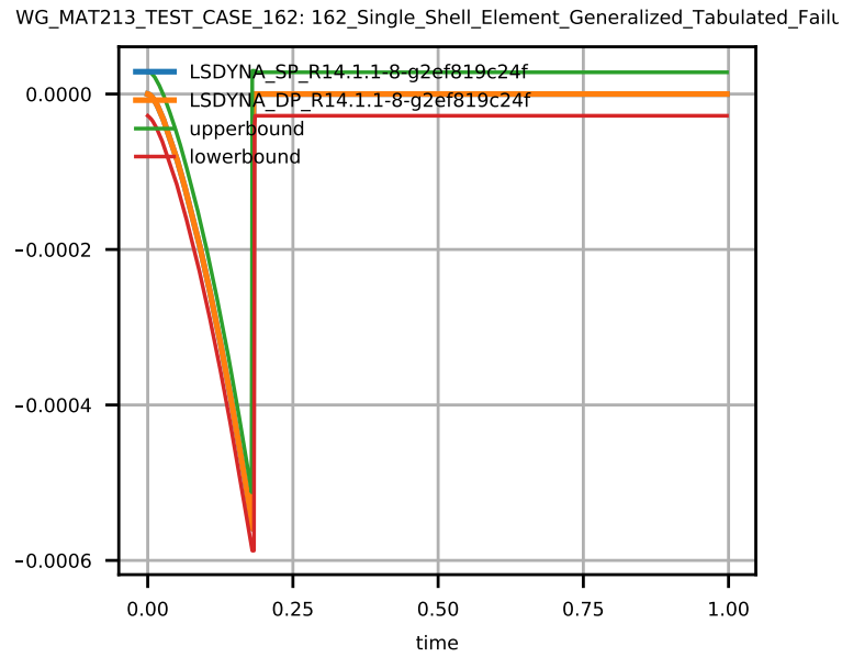
Figure 15: Shell Element Stress \sigma_{xy} at lower integration point in thickness.
