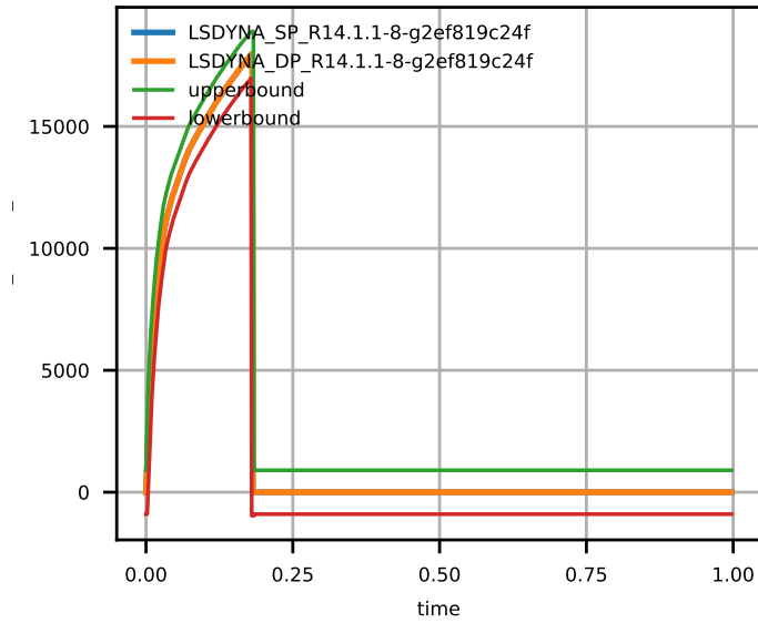
Figure 5: Shell Element Stress \sigma_y at integration point 2.
