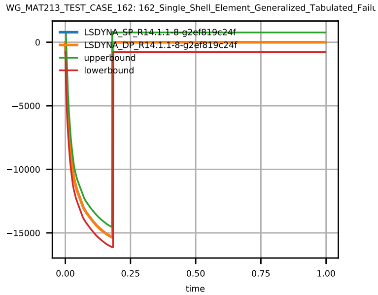
Figure 10: Shell Element Stress \sigma_{xx} at integration point 4.
