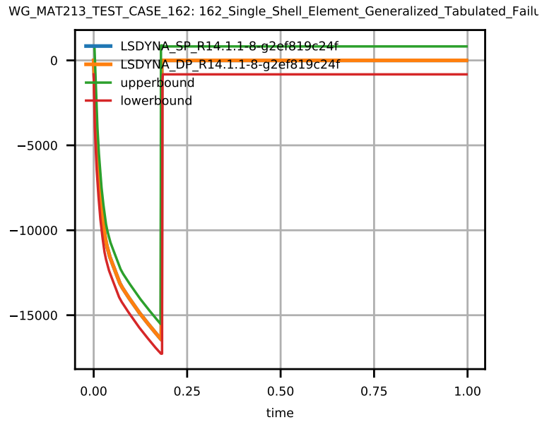
Figure 4: Shell Element Stress \sigma_{xx} at integration point 2.
