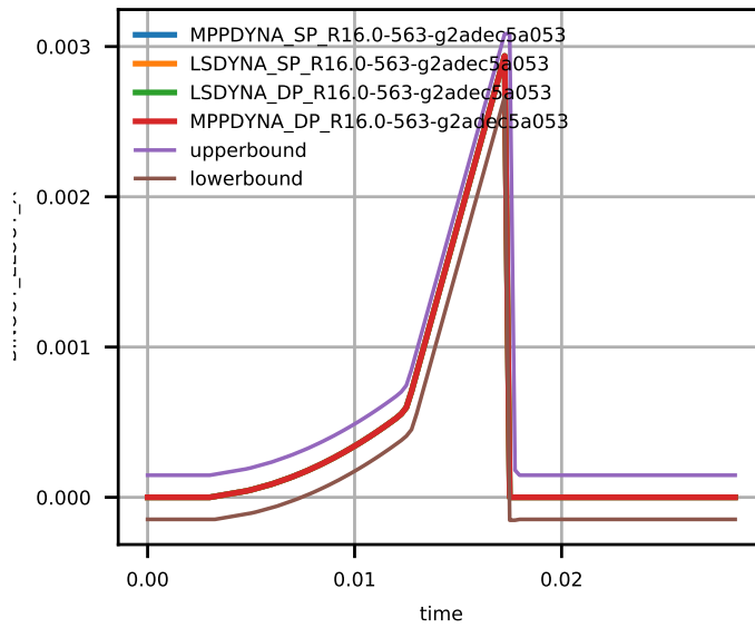
Figure 13: Solid Element Strain zx.
