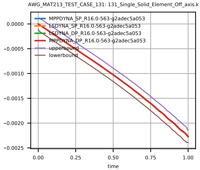
Figure 3: Solid Element Strain \epsilon_{zz} .
