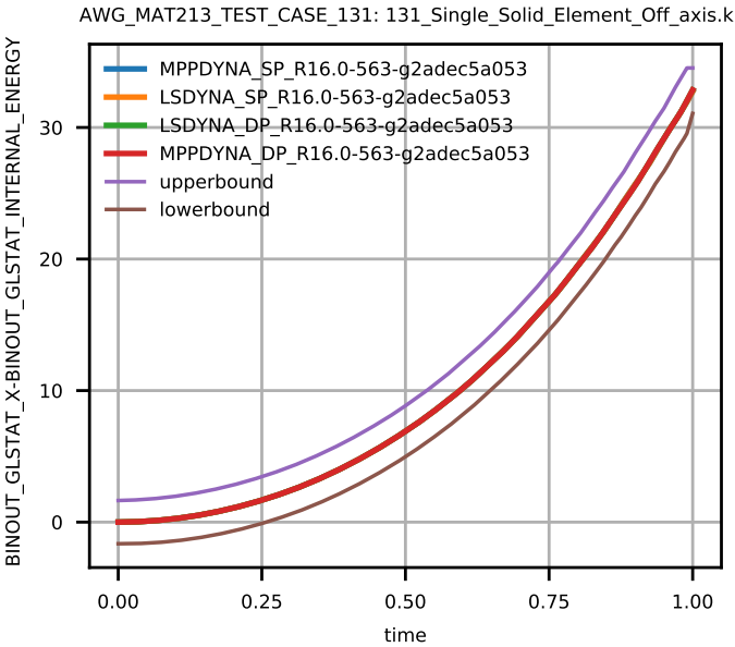
Figure 7: Global Internal Energy.
