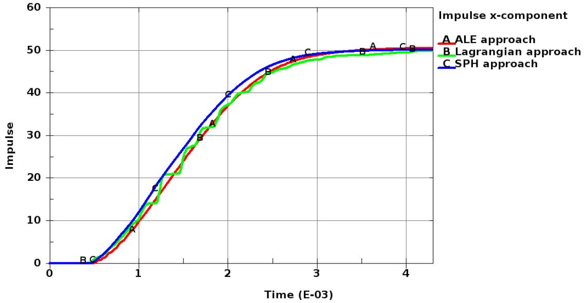
Figure 11: Platform averaged impulse for the different modelling approaches
