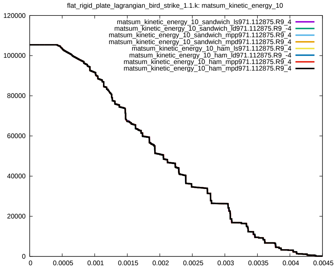
Figure 5: Cross platform results, kinetic energy part 10 (bird body), sub test case ID 1
