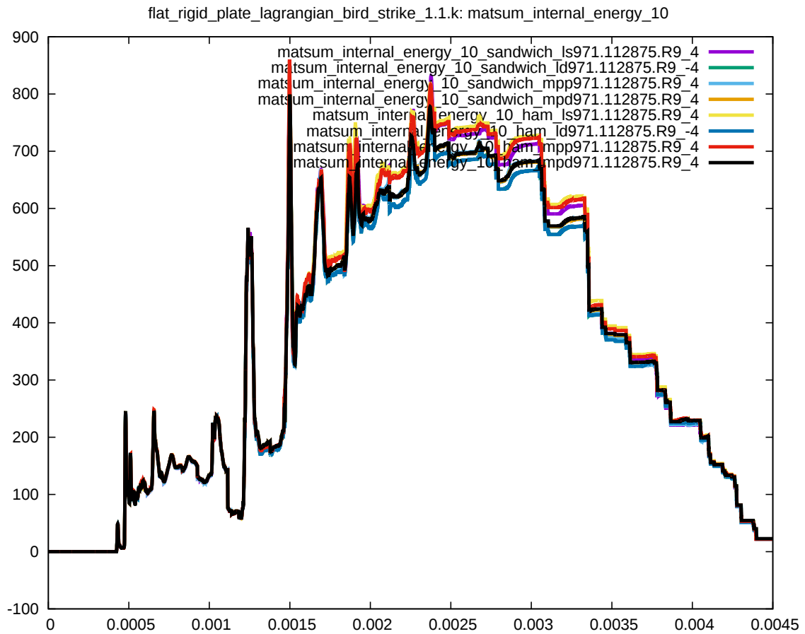
Figure 6: Cross platform results, internal energy part 10 (bird body), sub test case ID 1
