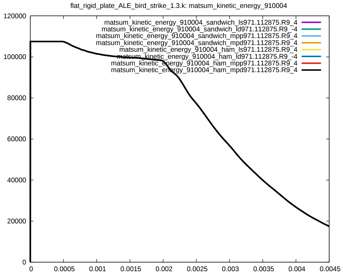
Figure 7: Cross platform results, kinetic energy part 910004 (bird body), sub test case ID 2
