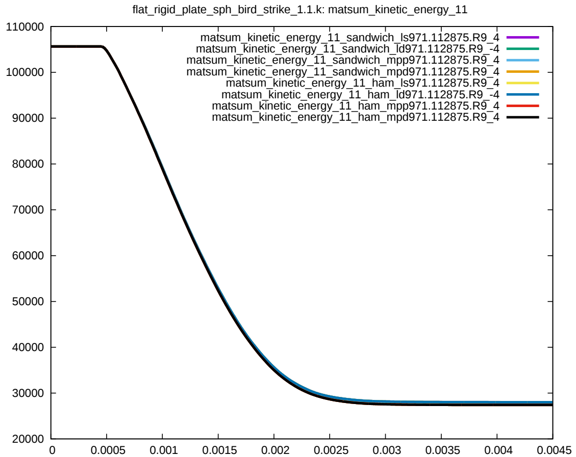
Figure 9: Cross platform results, kinetic energy part 11 (bird body), sub test case ID 3
