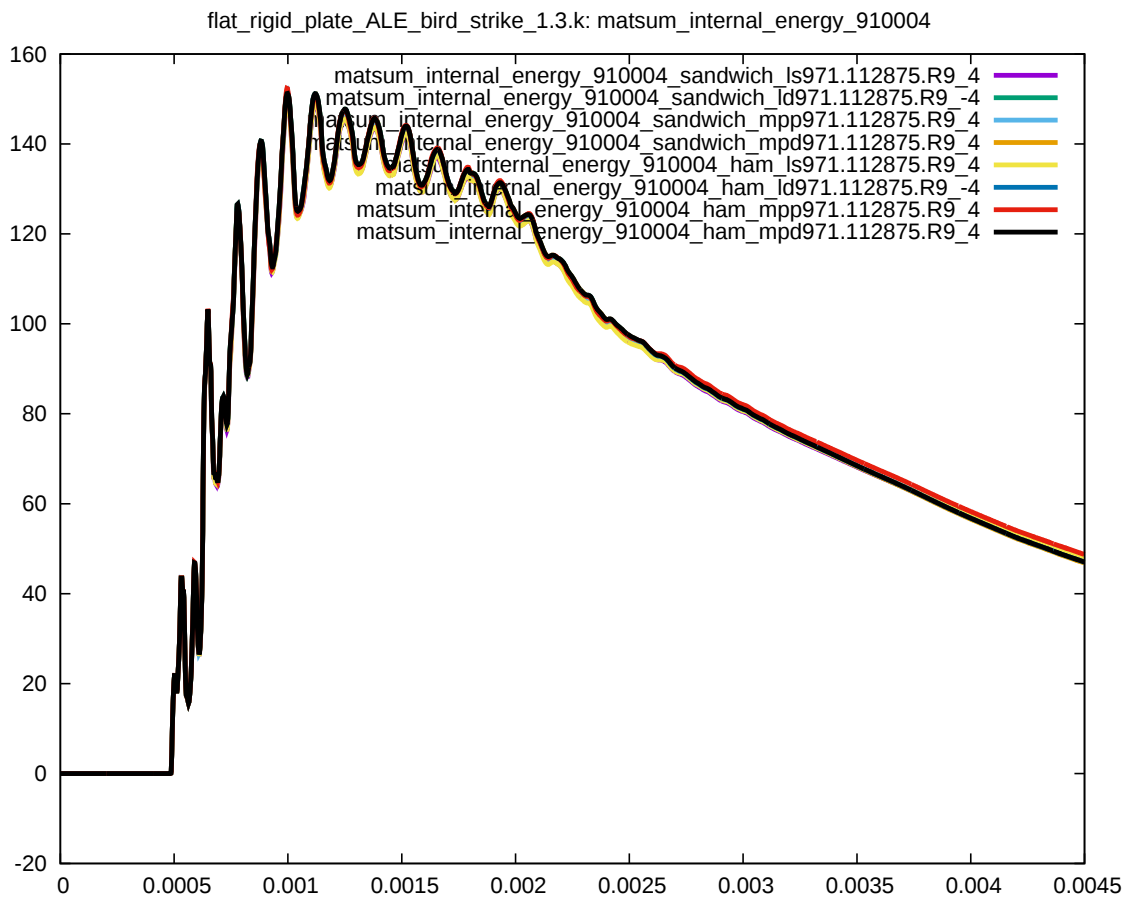
Figure 8: Cross platform results, internal energy part 920004 (bird body), sub test case ID 2
