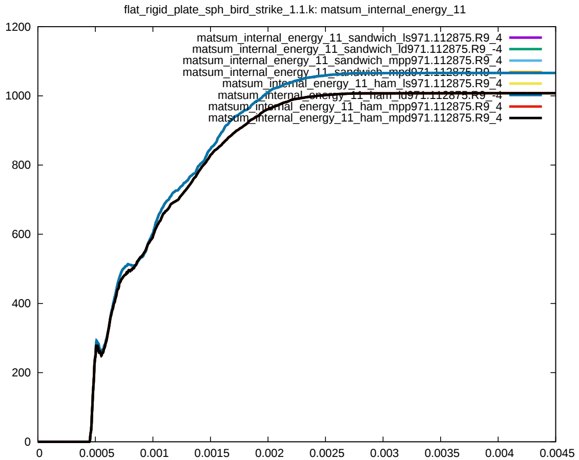
Figure 10: Cross platform results, internal energy part 11 (bird body), sub test case ID 3
