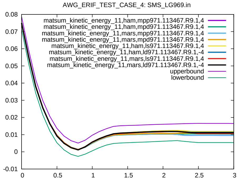
Figure 7: Cross platform results, kinetic energy part 11, sub test case ID 4
