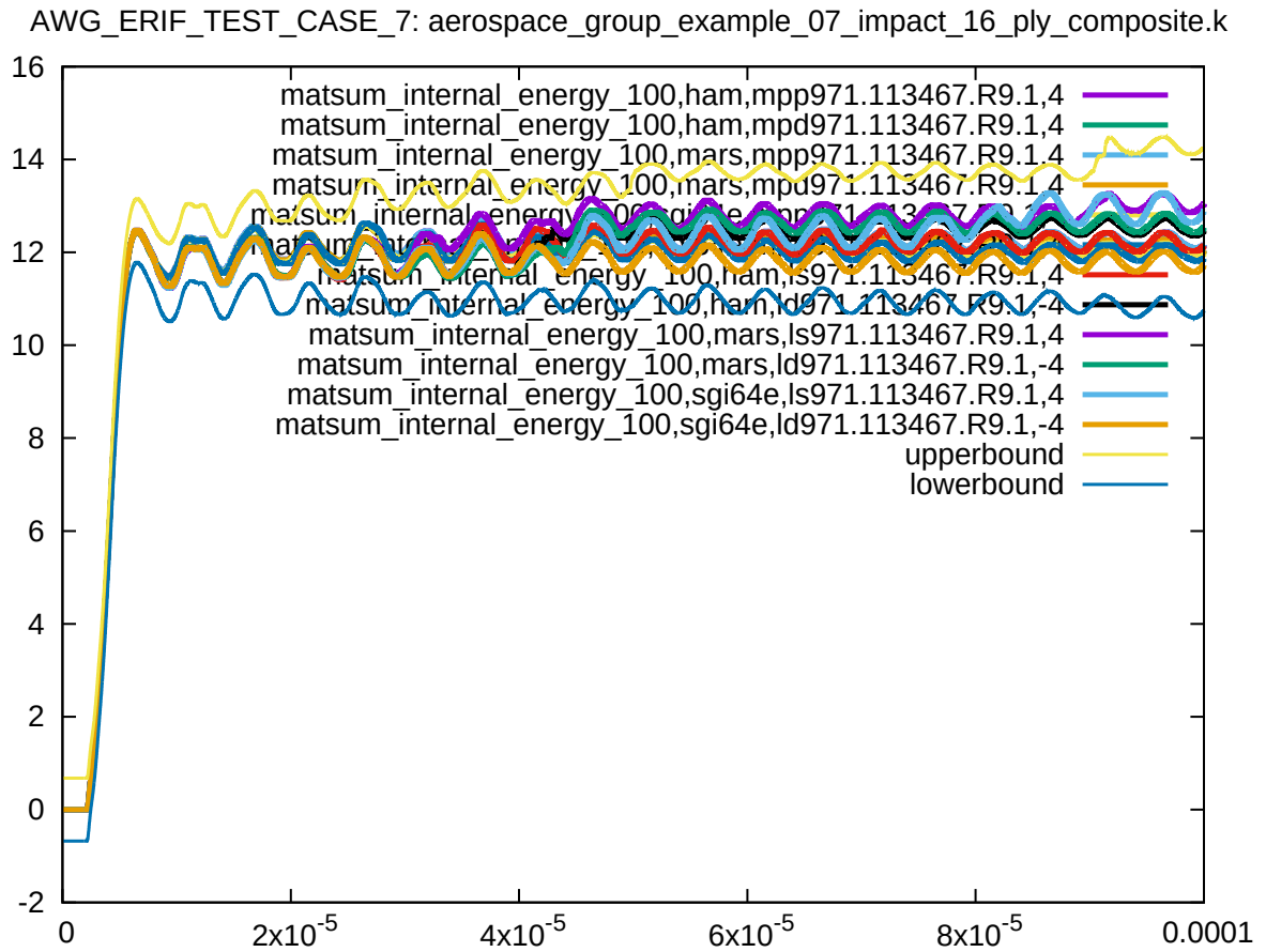
Figure 6: Cross platform results, internal energy part 100, sub test case ID 1
