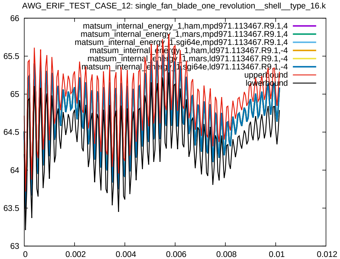
Figure 5: Cross platform results, internal energy part 1, sub test case ID 2
