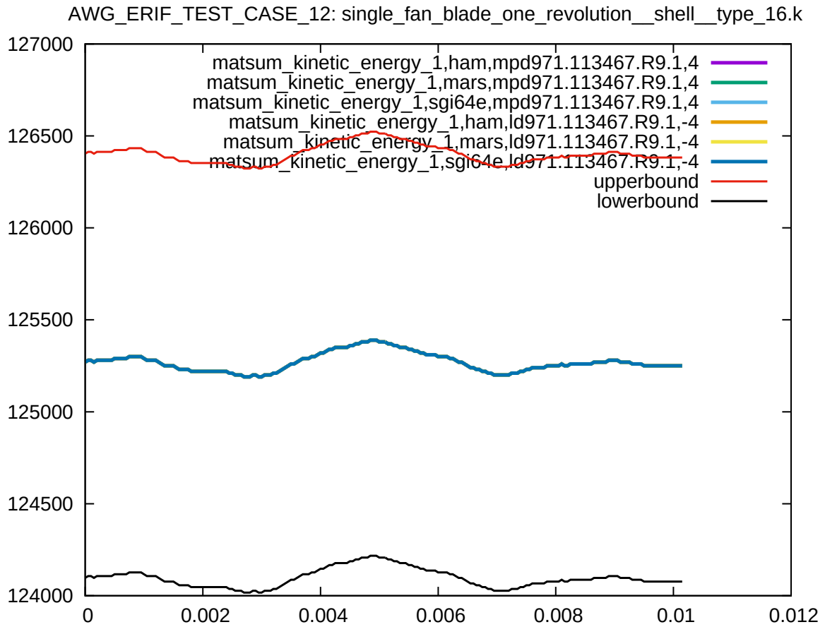
Figure 6: Cross platform results, kinetic energy part 1, sub test case ID 2
