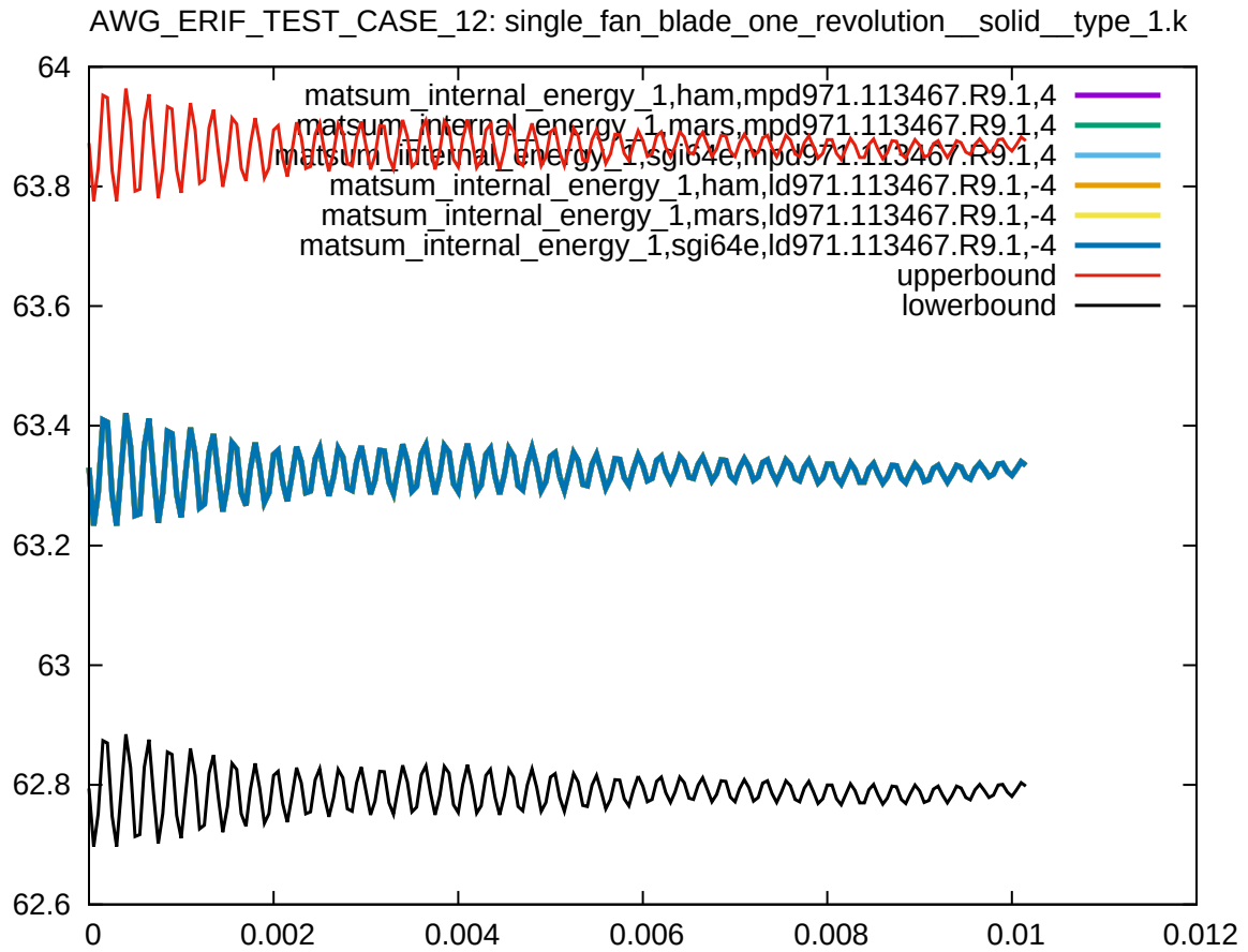
Figure 3: Cross platform results, internal energy part 1, sub test case ID 1
