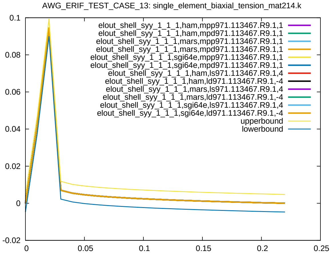
Figure 10: Cross platform results, stress in y-direction, integration point 1, sub test case ID 6
