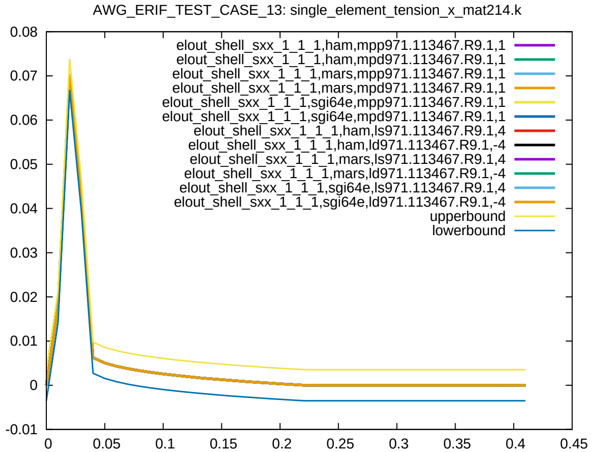
Figure 3: Cross platform results, stress in x-direction, integration point 1, sub test case ID 1
