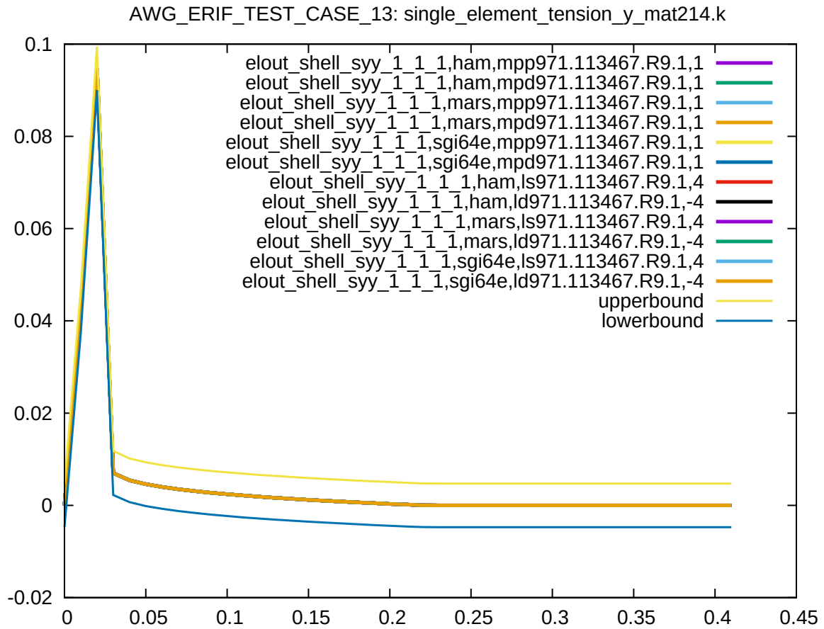
Figure 4: Cross platform results, stress in y-direction, integration point 1, sub test case ID 2
