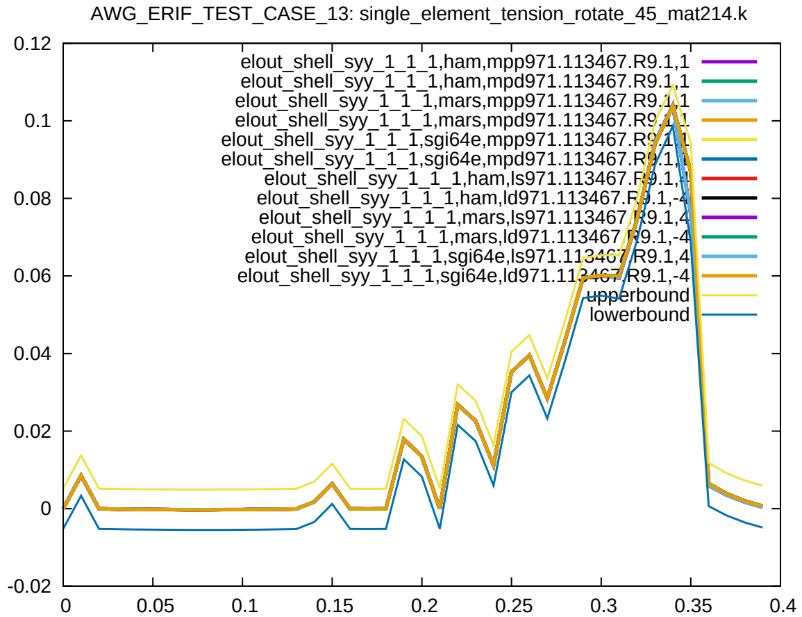
Figure 8: Cross platform results, stress in y-direction, integration point 1, sub test case ID 5
