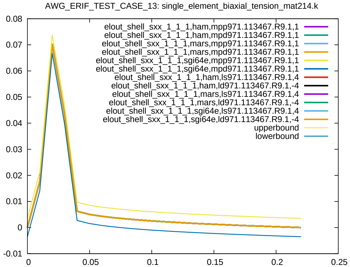
Figure 9: Cross platform results, stress in x-direction, integration point 1, sub test case ID 6
