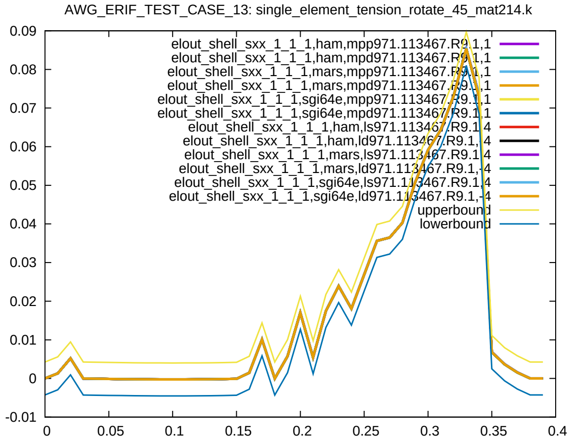
Figure 7: Cross platform results, stress in x-direction, integration point 1, sub test case ID 5
