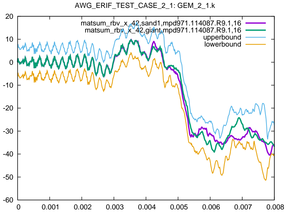
Figure 6: Rigid body velocity (x-component) part 42 (released blade), sub test case ID 1
