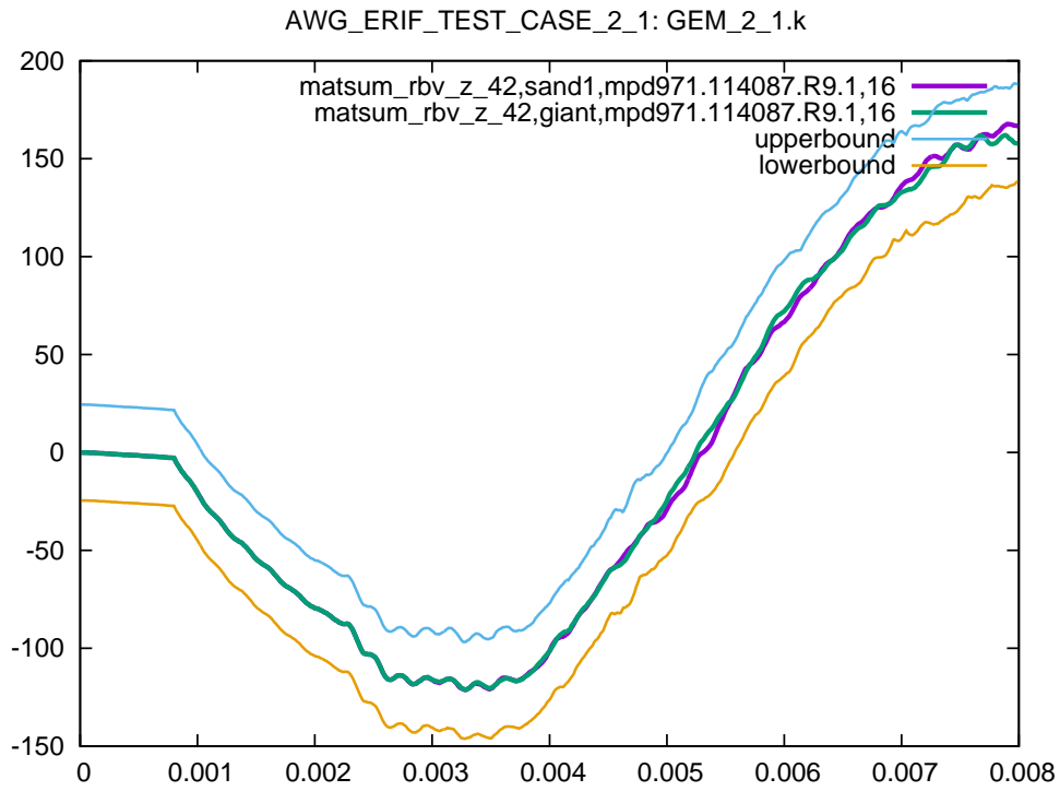
Figure 8: Rigid body velocity (z-component) part 42 (released blade), sub test case ID 1
