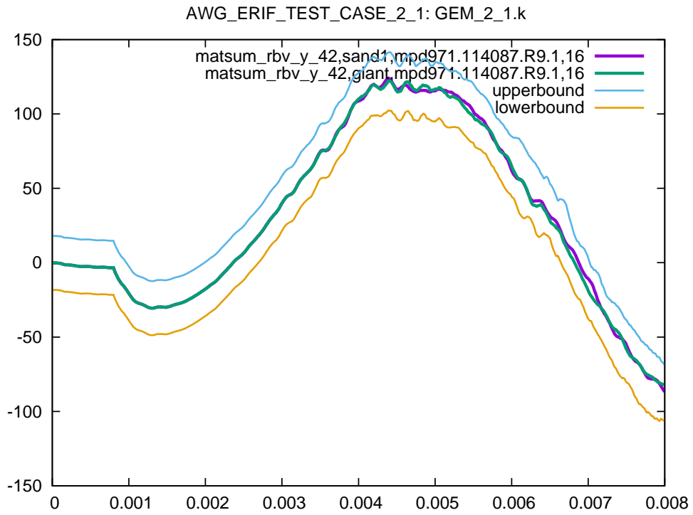
Figure 7: Rigid body velocity (y-component) part 42 (released blade), sub test case ID 1
