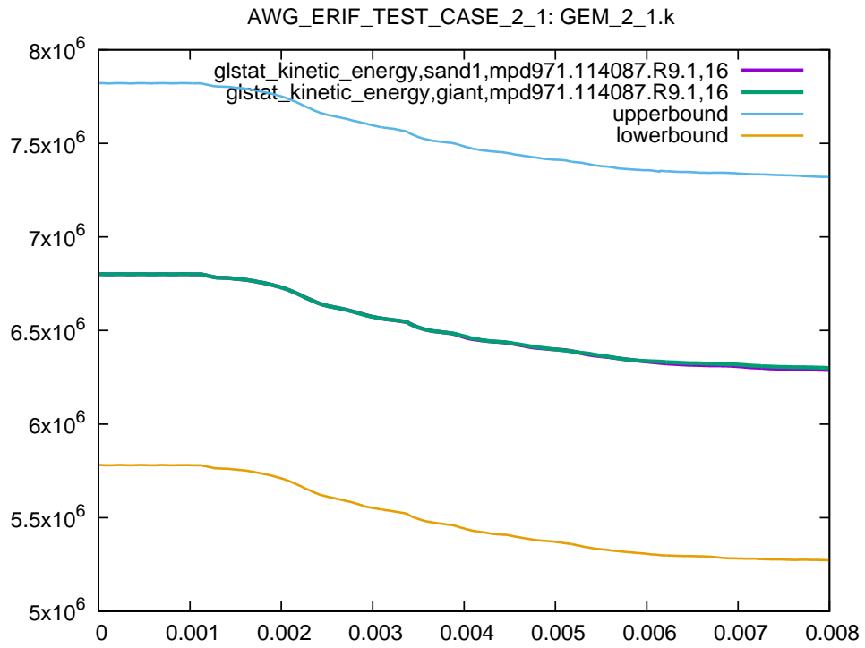
Figure 3: Global kinetic energy, sub test case ID 1
