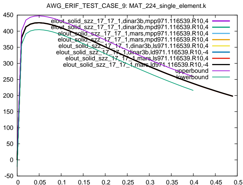
Figure 19: Cross platform results, zz stress element id 17, sub test case ID 1
