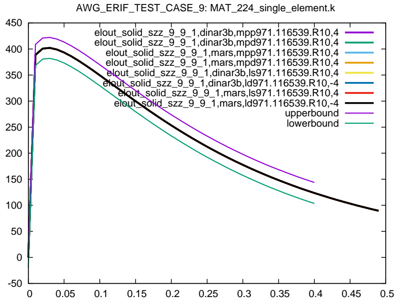
Figure 11: Cross platform results, zz stress element id 9, sub test case ID 1
