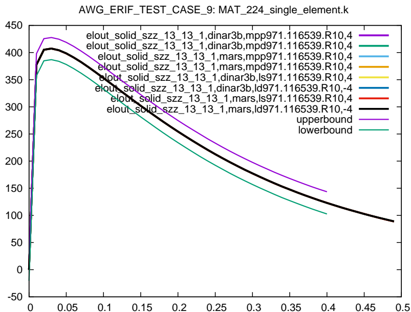
Figure 15: Cross platform results, zz stress element id 13, sub test case ID 1
