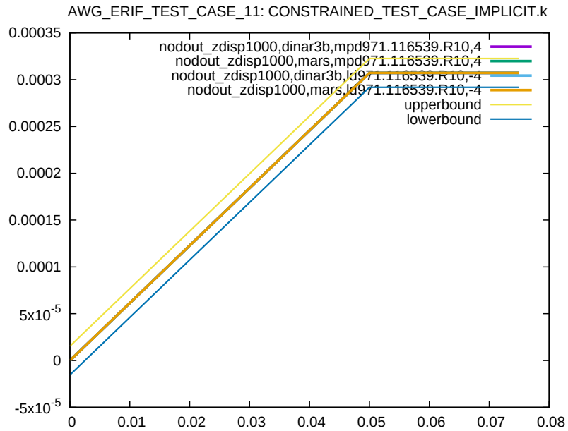
Figure 17: Cross platform results, nodal displacement in z-direction, node 1000, sub test case ID 2
