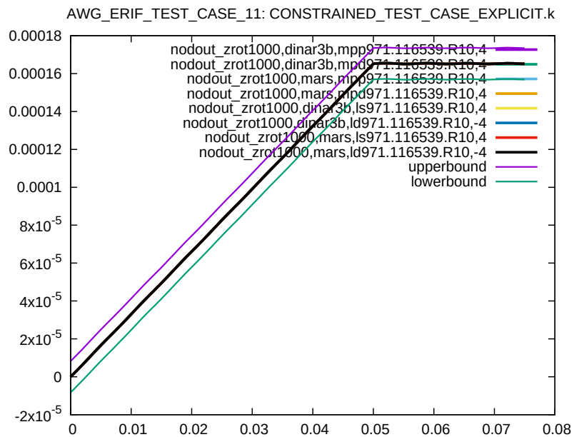
Figure 8: Cross platform results, nodal rotation around z-axis, node 1000, sub test case ID 1
