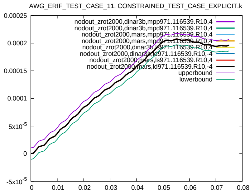
Figure 14: Cross platform results, nodal rotation around z-axis, node 2000, sub test case ID 1
