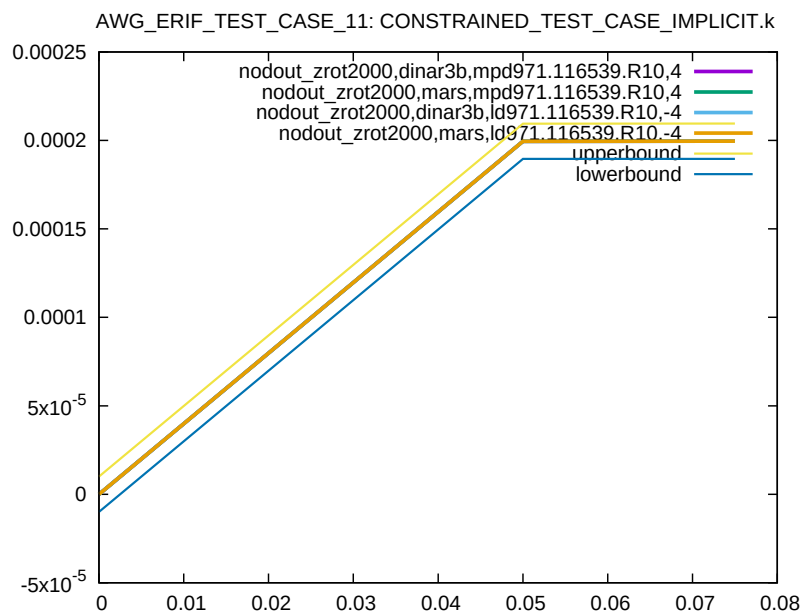
Figure 26: Cross platform results, nodal rotation around z-axis, node 2000, sub test case ID 2
