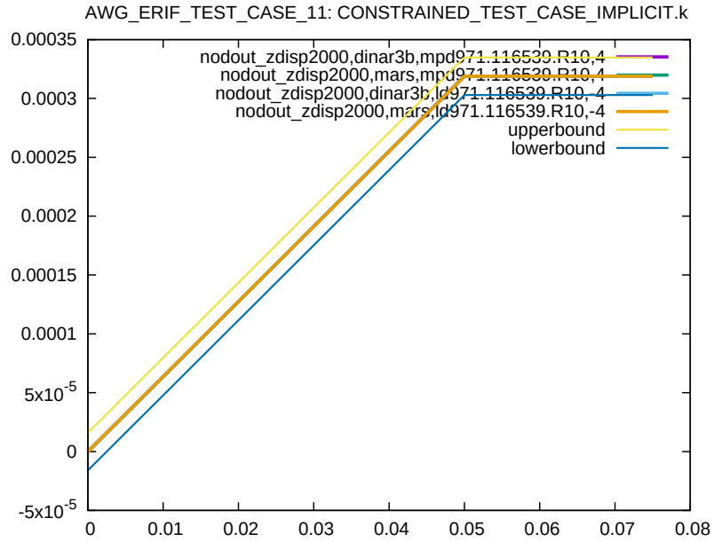
Figure 23: Cross platform results, nodal displacement in z-direction, node 2000, sub test case ID 2
