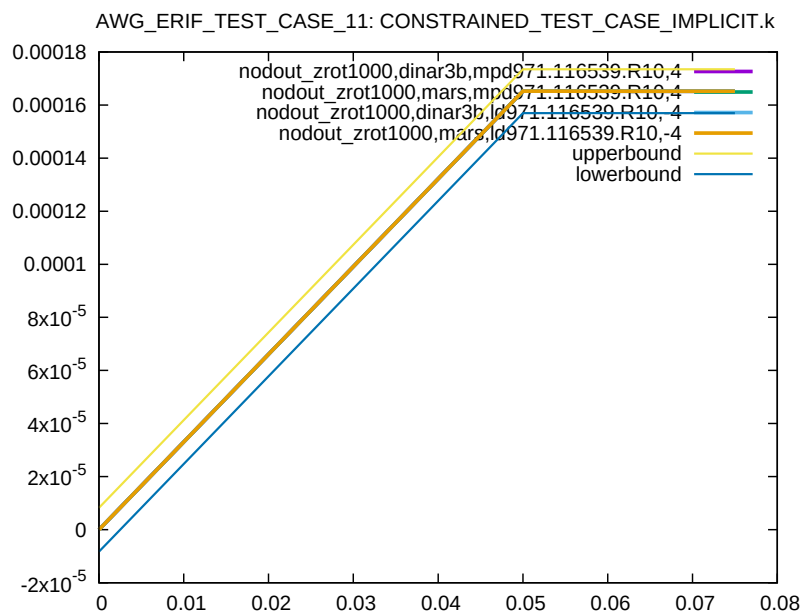
Figure 20: Cross platform results, nodal rotation around z-axis, node 1000, sub test case ID 2
