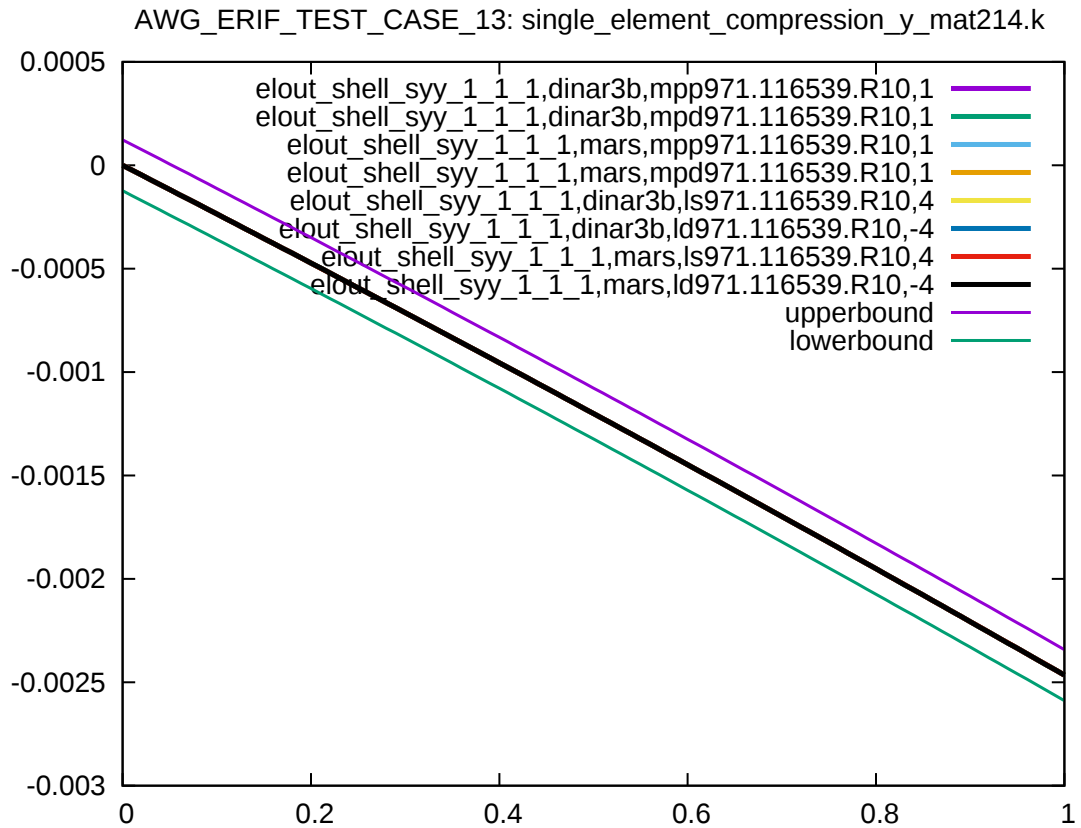
Figure 6: Cross platform results, stress in y-direction, integration point 1, sub test case ID 4
