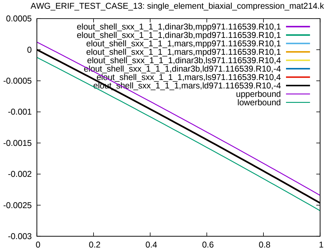
Figure 13: Cross platform results, stress in x-direction, integration point 1, sub test case ID 8
