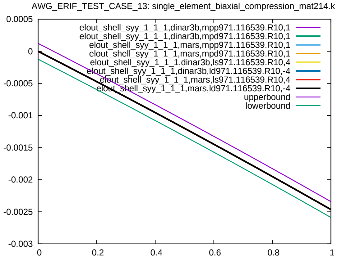
Figure 14: Cross platform results, stress in y-direction, integration point 1, sub test case ID 8
