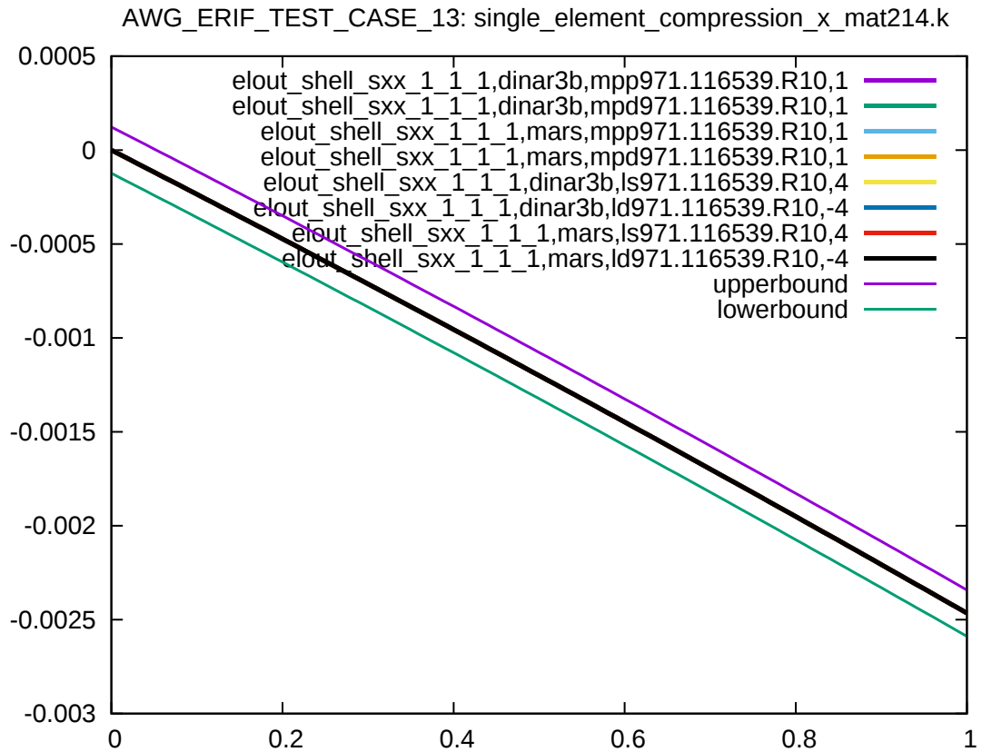
Figure 5: Cross platform results, stress in x-direction, integration point 1, sub test case ID 3
