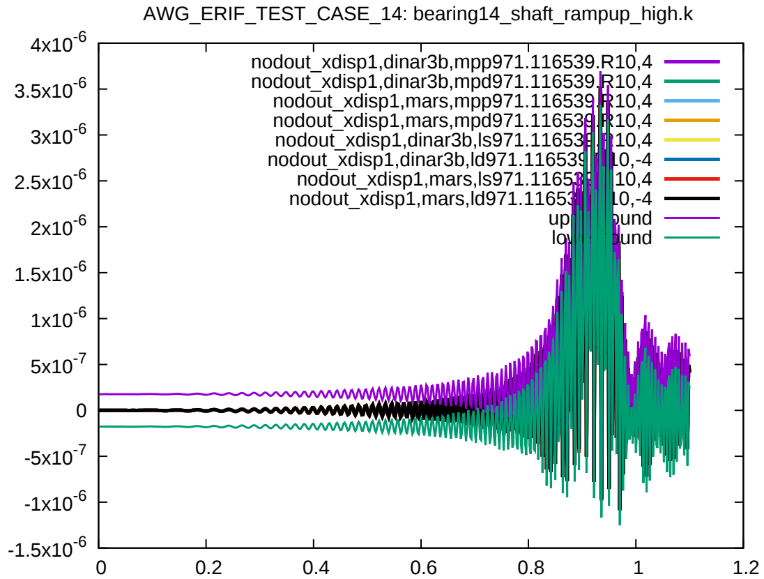
Figure 1: Cross platform results, node displacement in x-direction, node id 1, sub test case ID 1
