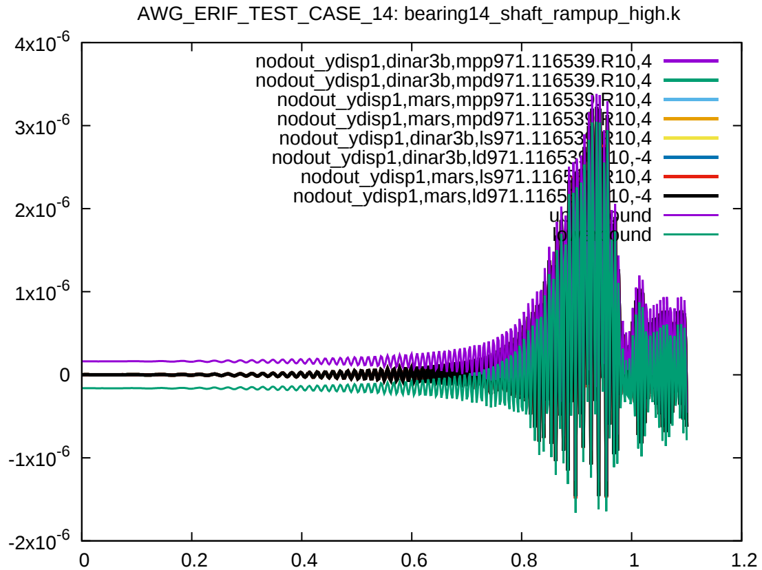
Figure 2: Cross platform results, node displacement in y-direction, node id 1, sub test case ID 1
