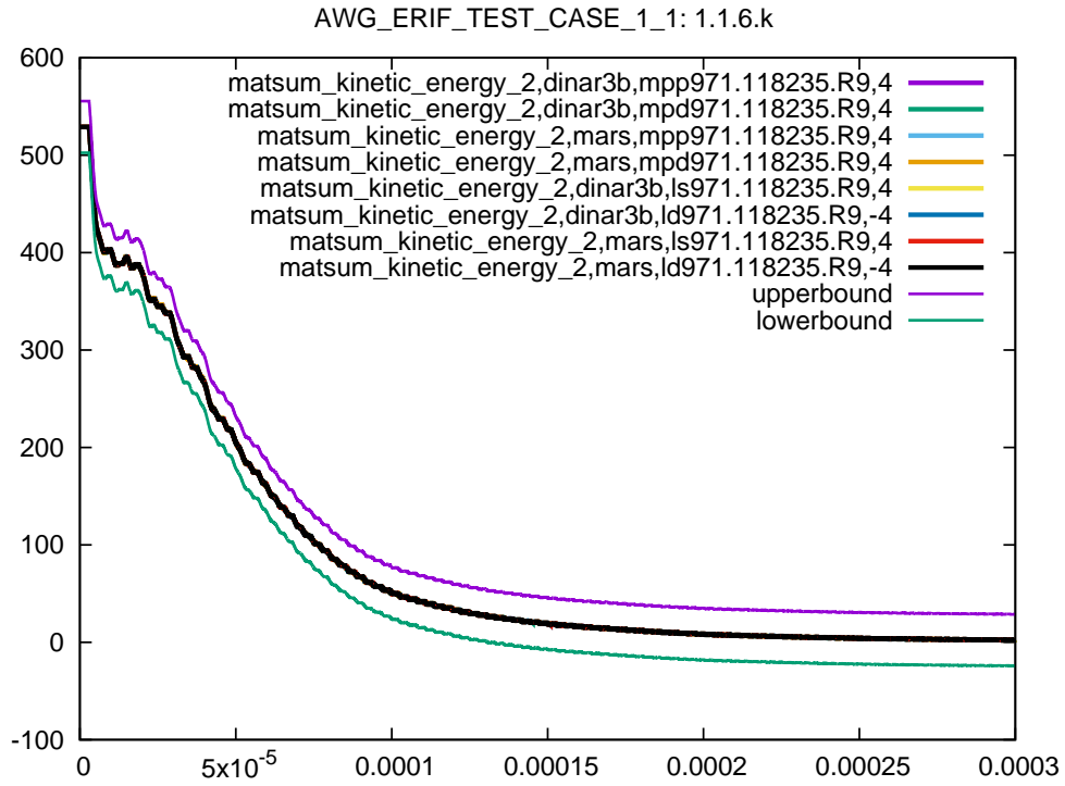
Figure 48: Cross platform results, kinetic energy part 2, sub test case ID 6, 95% ballistic limit
