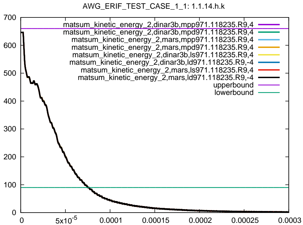
Figure 42: Cross platform results, kinetic energy part 2, sub test case ID 14, 105% ballistic limit
