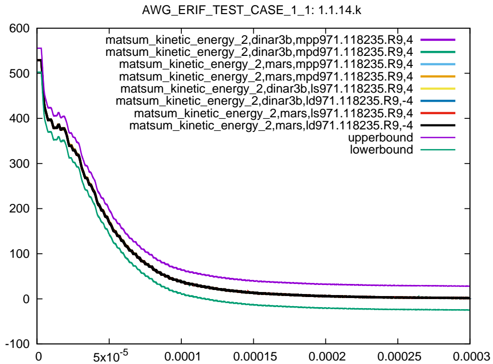
Figure 55: Cross platform results, kinetic energy part 2, sub test case ID 14, 95% ballistic limit
