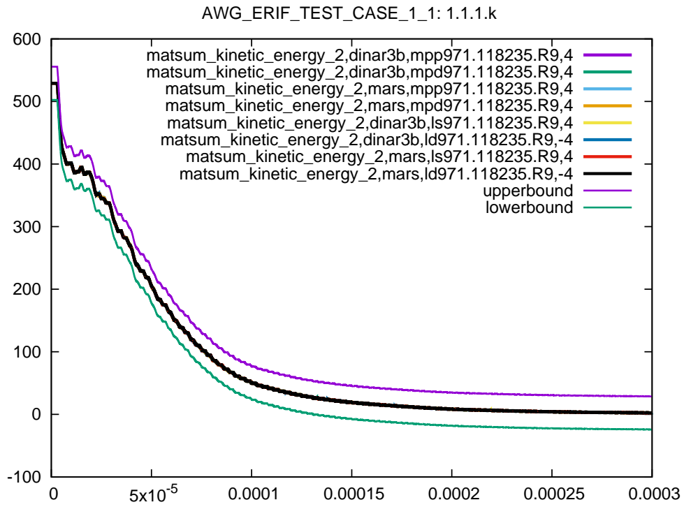
Figure 43: Cross platform results, kinetic energy part 2, sub test case ID 1, 95% ballistic limit
