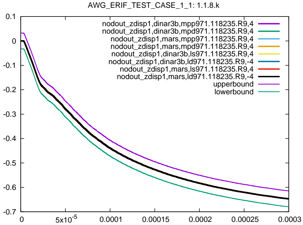
Figure 24: Cross platform results, nodal z displacement node 1, sub test case ID 8, 95% ballistic limit
