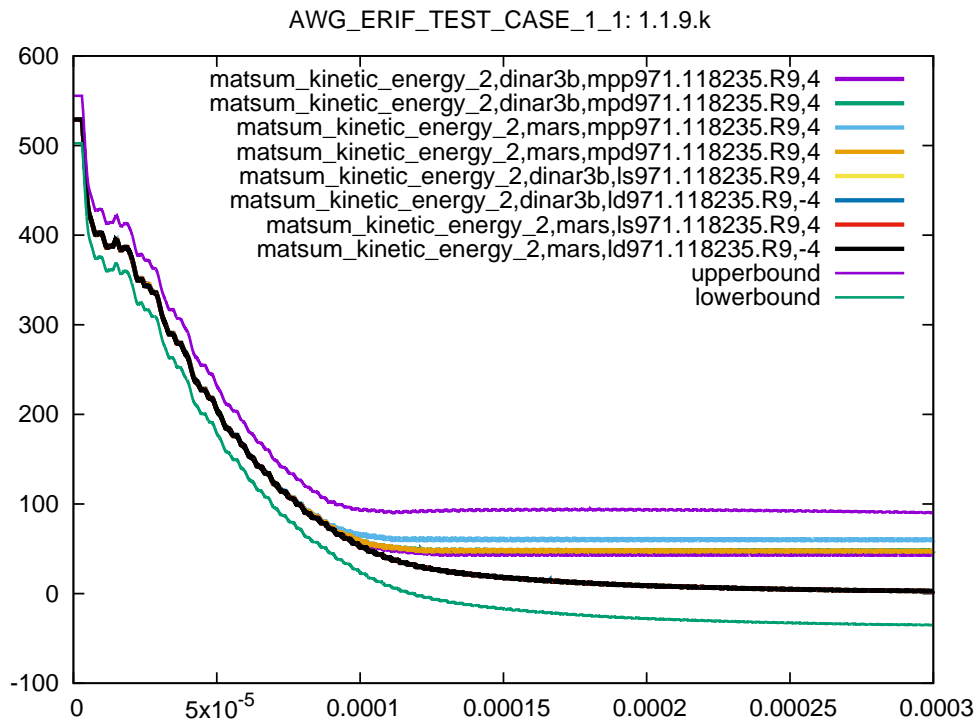
Figure 51: Cross platform results, kinetic energy part 2, sub test case ID 9, 95% ballistic limit
