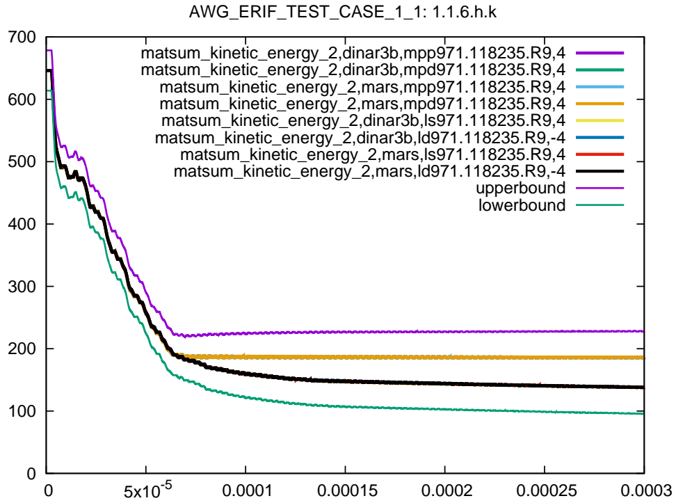
Figure 35: Cross platform results, kinetic energy part 2, sub test case ID 6, 105% ballistic limit
