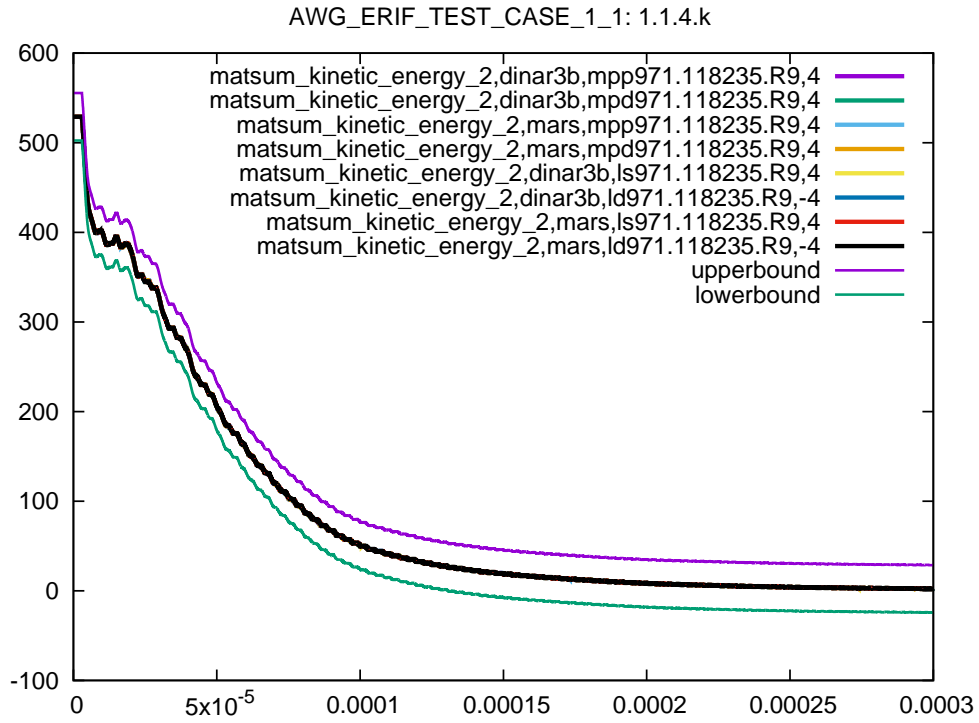
Figure 46: Cross platform results, kinetic energy part 2, sub test case ID 4, 95% ballistic limit
