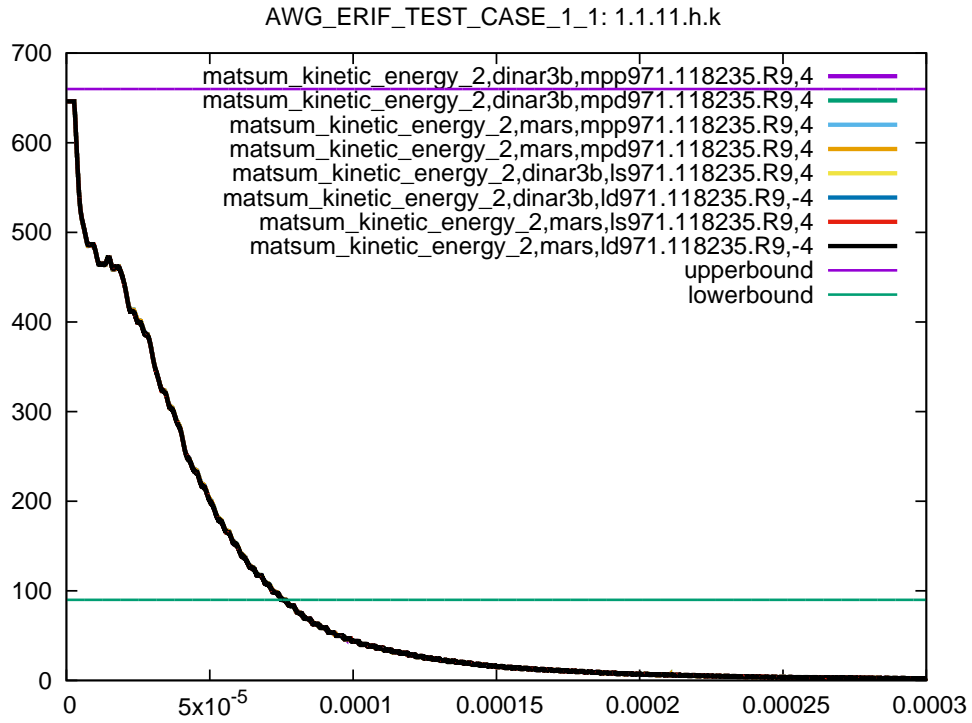
Figure 39: Cross platform results, kinetic energy part 2, sub test case ID 11, 105% ballistic limit
