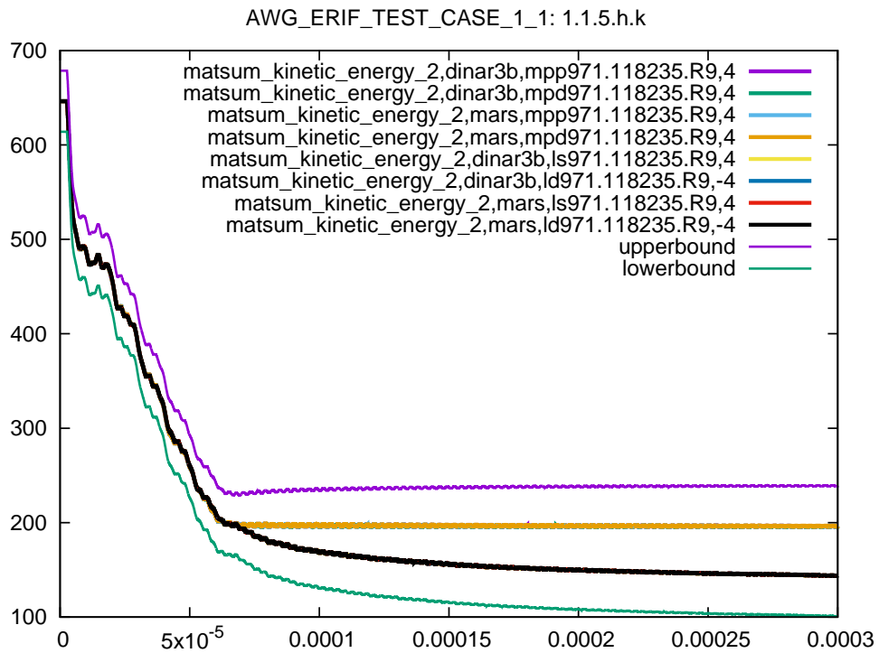
Figure 34: Cross platform results, kinetic energy part 2, sub test case ID 5, 105% ballistic limit
