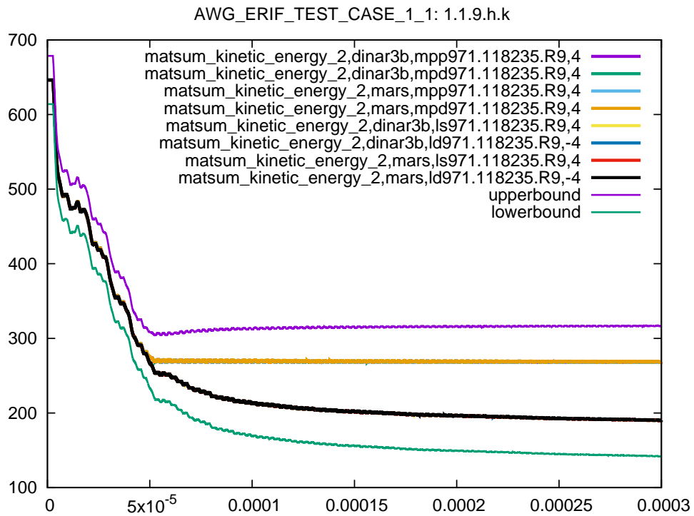
Figure 38: Cross platform results, kinetic energy part 2, sub test case ID 9, 105% ballistic limit
