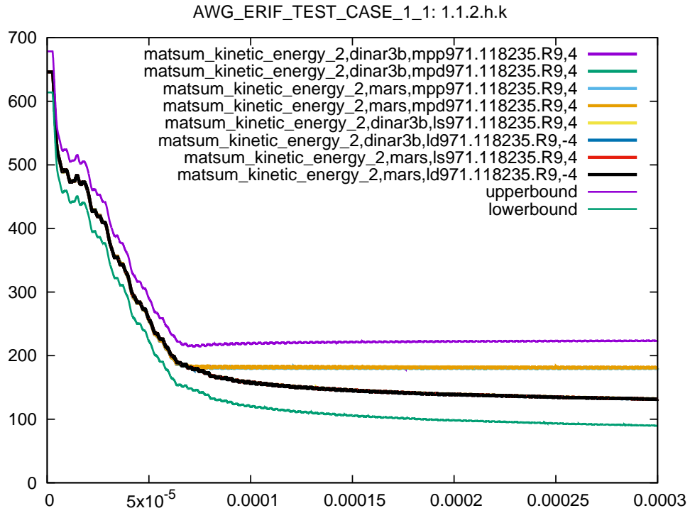
Figure 31: Cross platform results, kinetic energy part 2, sub test case ID 2, 105% ballistic limit
