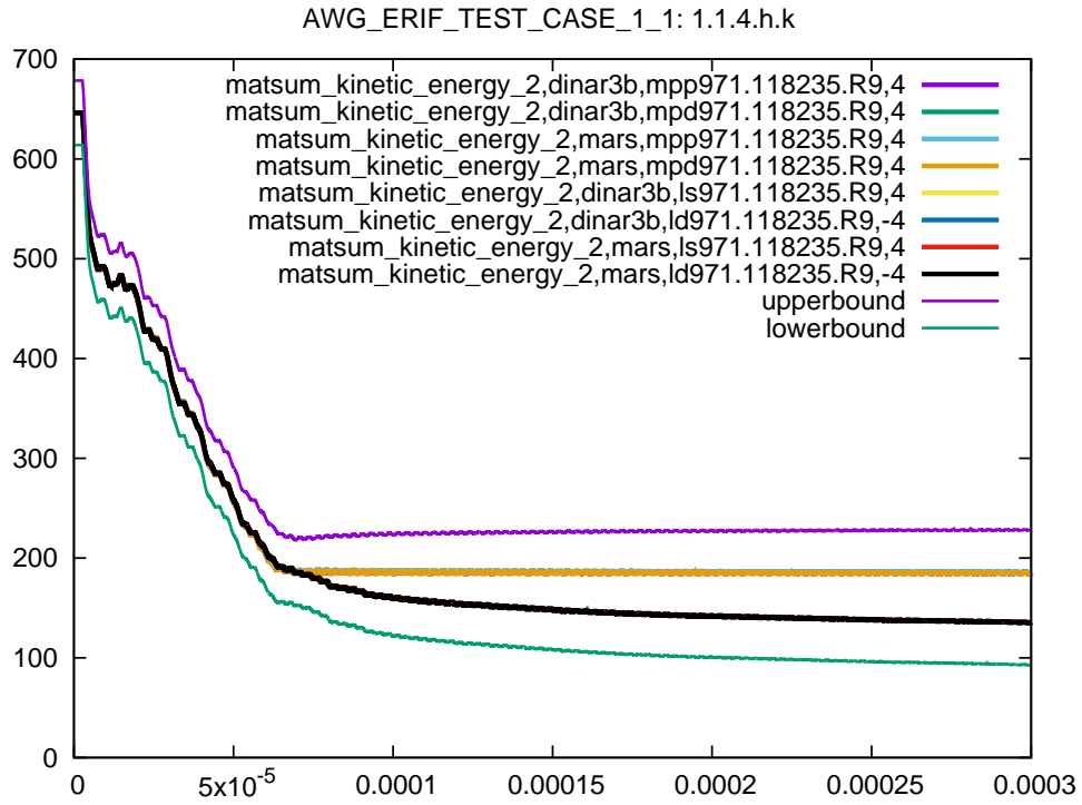
Figure 33: Cross platform results, kinetic energy part 2, sub test case ID 4, 105% ballistic limit
