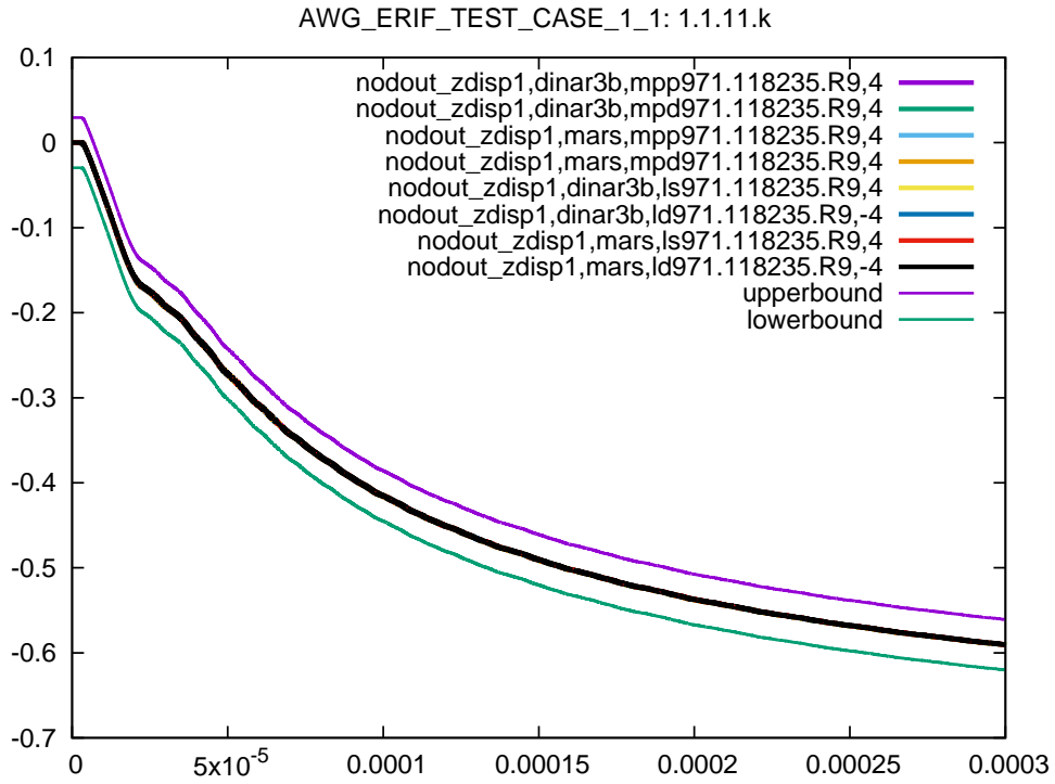
Figure 26: Cross platform results, nodal z displacement node 1, sub test case ID 11, 95% ballistic limit
