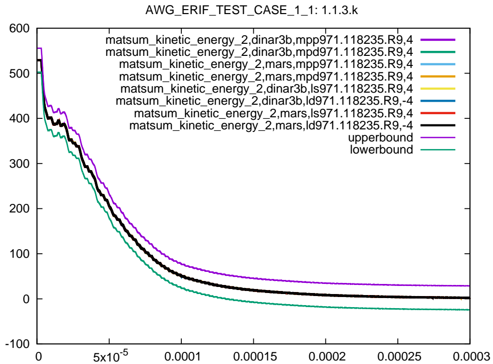
Figure 45: Cross platform results, kinetic energy part 2, sub test case ID 3, 95% ballistic limit
