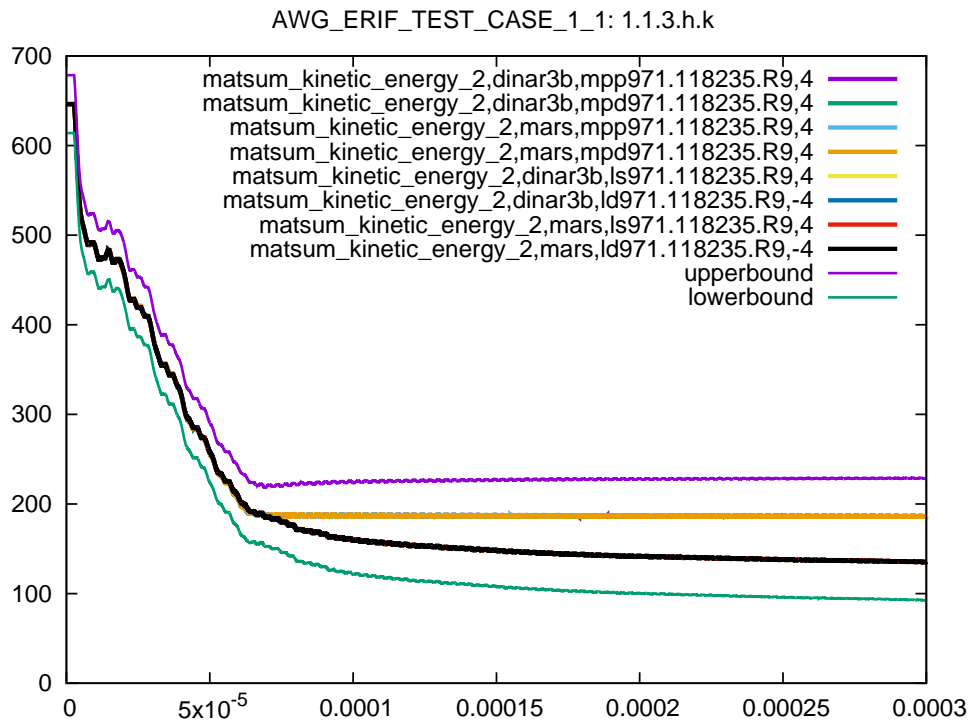
Figure 32: Cross platform results, kinetic energy part 2, sub test case ID 3, 105% ballistic limit
