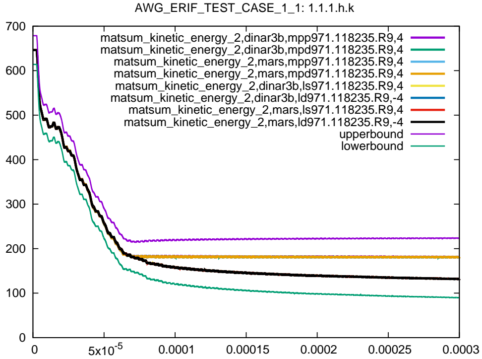
Figure 30: Cross platform results, kinetic energy part 2, sub test case ID 1, 105% ballistic limit
