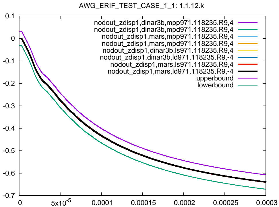
Figure 27: Cross platform results, nodal z displacement node 1, sub test case ID 12, 95% ballistic limit
