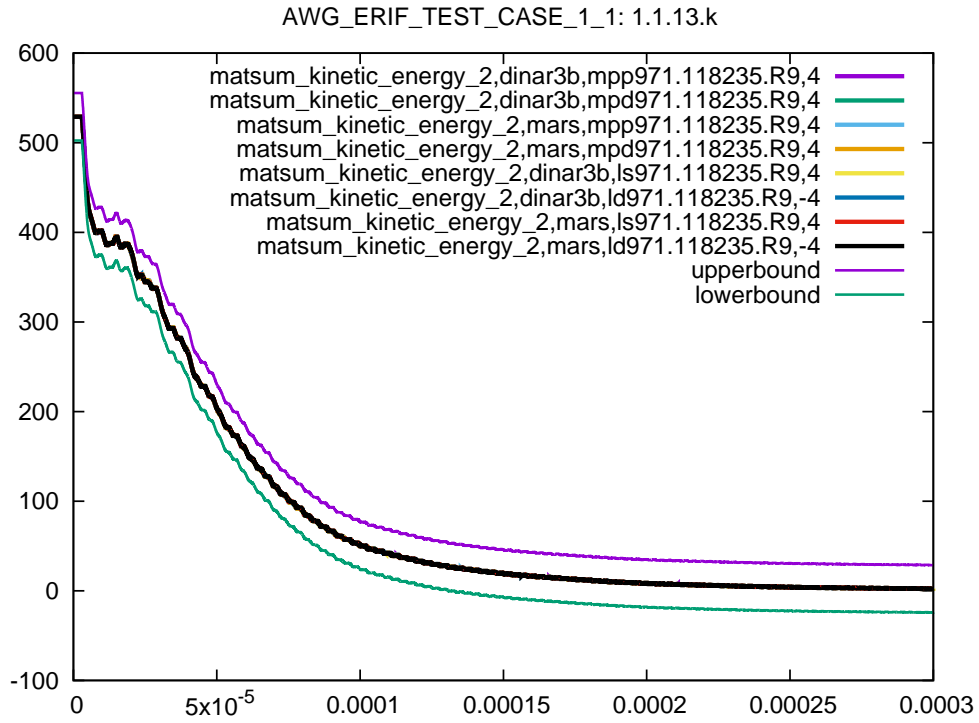
Figure 54: Cross platform results, kinetic energy part 2, sub test case ID 13, 95% ballistic limit
