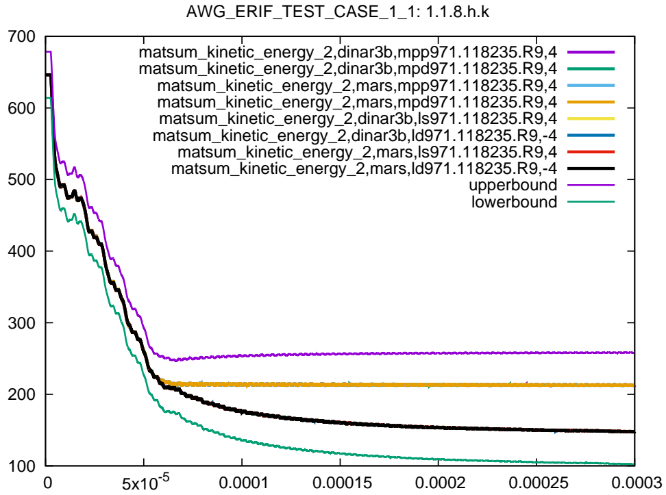
Figure 37: Cross platform results, kinetic energy part 2, sub test case ID 8, 105% ballistic limit
