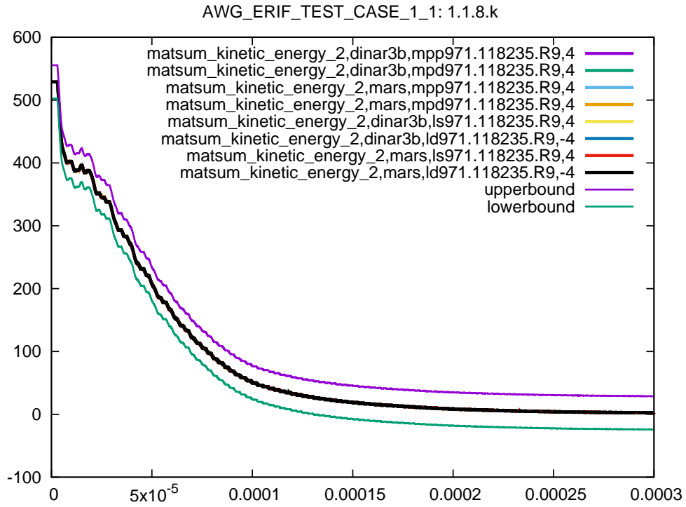
Figure 50: Cross platform results, kinetic energy part 2, sub test case ID 8
