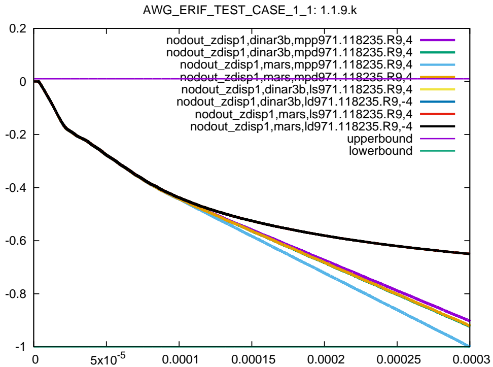
Figure 25: Cross platform results, nodal z displacement node 1, sub test case ID 9, 95% ballistic limit
