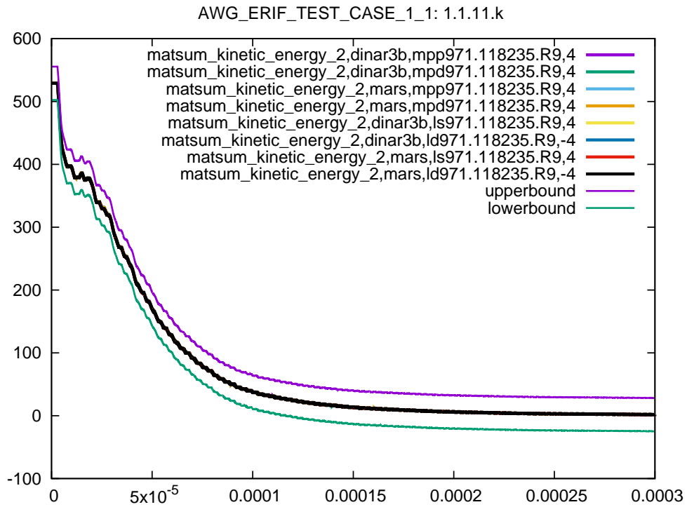
Figure 52: Cross platform results, kinetic energy part 2, sub test case ID 11, 95% ballistic limit
