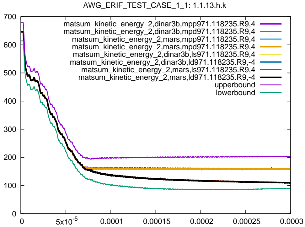
Figure 41: Cross platform results, kinetic energy part 2, sub test case ID 13, 105% ballistic limit
