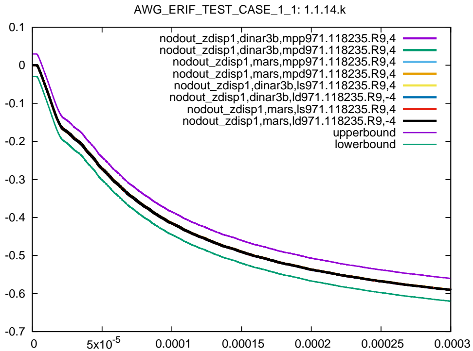
Figure 29: Cross platform results, nodal z displacement node 1, sub test case ID 14, 95% ballistic limit
