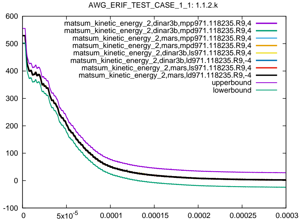
Figure 44: Cross platform results, kinetic energy part 2, sub test case ID 2, 95% ballistic limit
