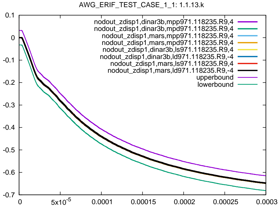
Figure 28: Cross platform results, nodal z displacement node 1, sub test case ID 13, 95% ballistic limit
