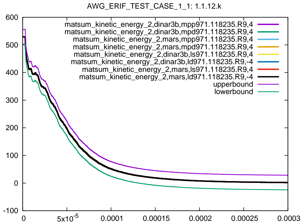
Figure 53: Cross platform results, kinetic energy part 2, sub test case ID 12, 95% ballistic limit
