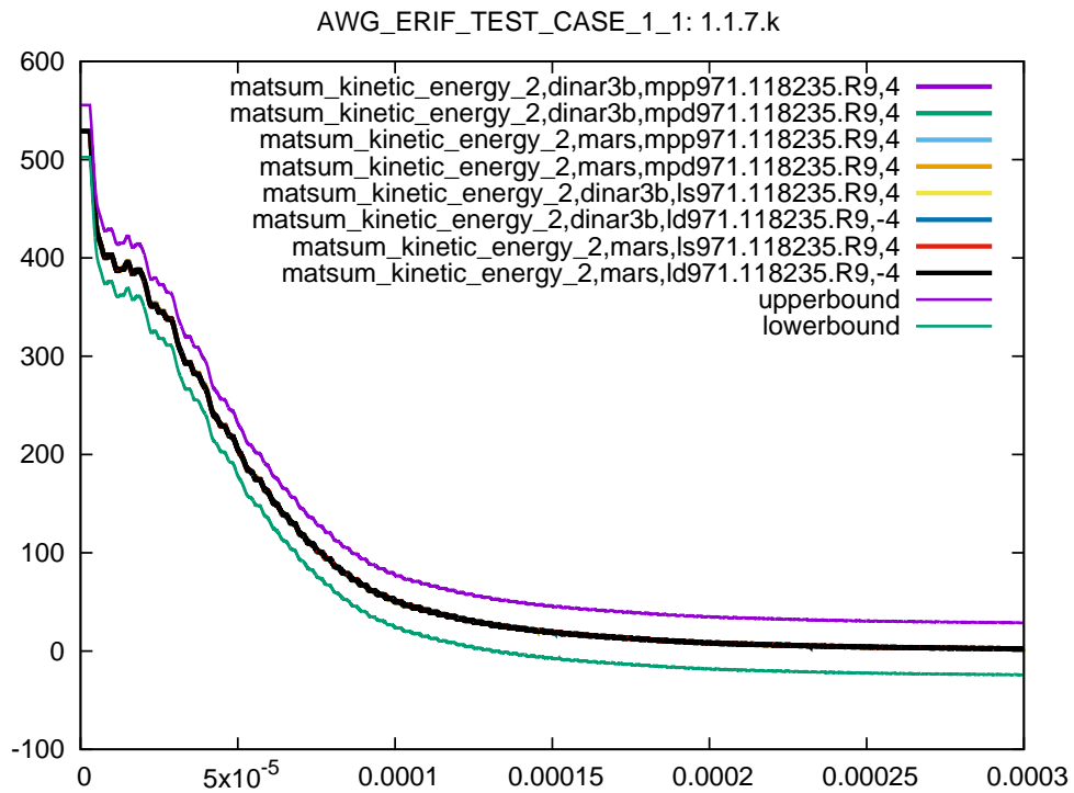
Figure 49: Cross platform results, kinetic energy part 2, sub test case ID 7, 95% ballistic limit
