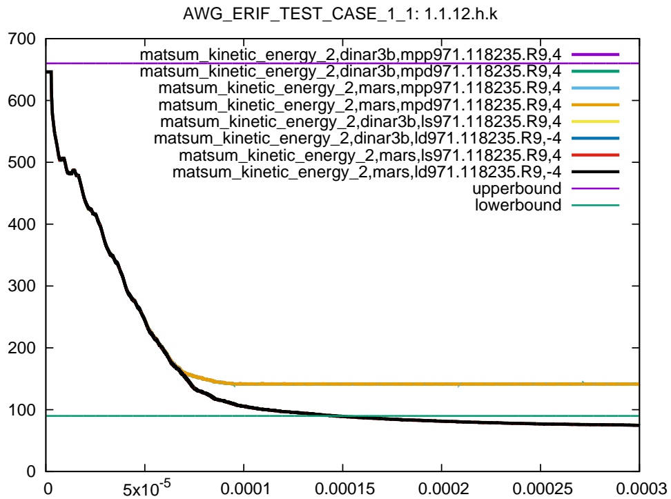
Figure 40: Cross platform results, kinetic energy part 2, sub test case ID 12, 105% ballistic limit
