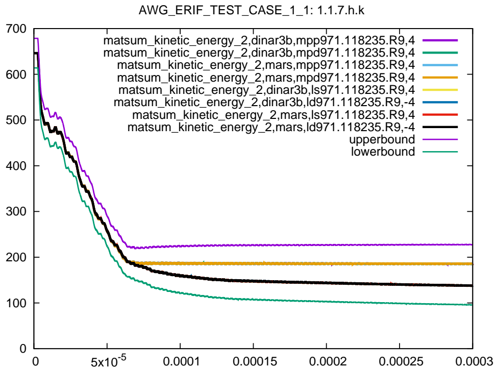
Figure 36: Cross platform results, kinetic energy part 2, sub test case ID 7, 105% ballistic limit
