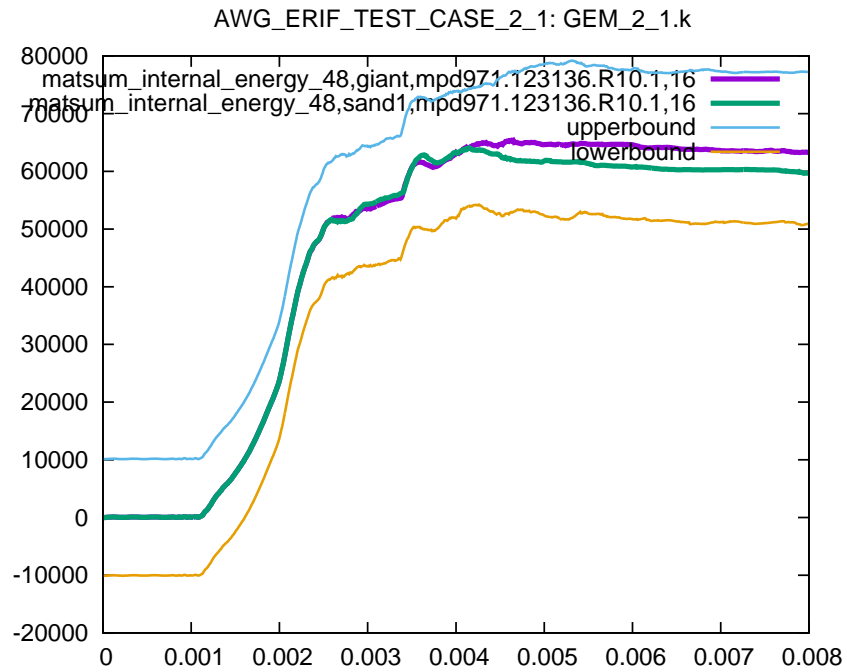
Figure 4: Internal energy part 48 (released blade), sub test case ID 1
