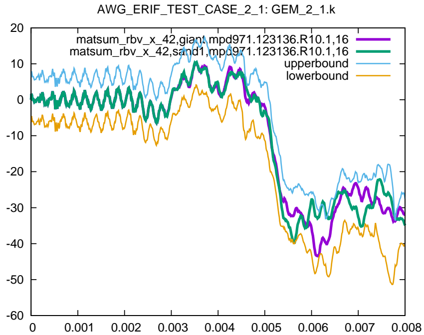
Figure 6: Rigid body velocity (x-component) part 42 (released blade), sub test case ID 1
