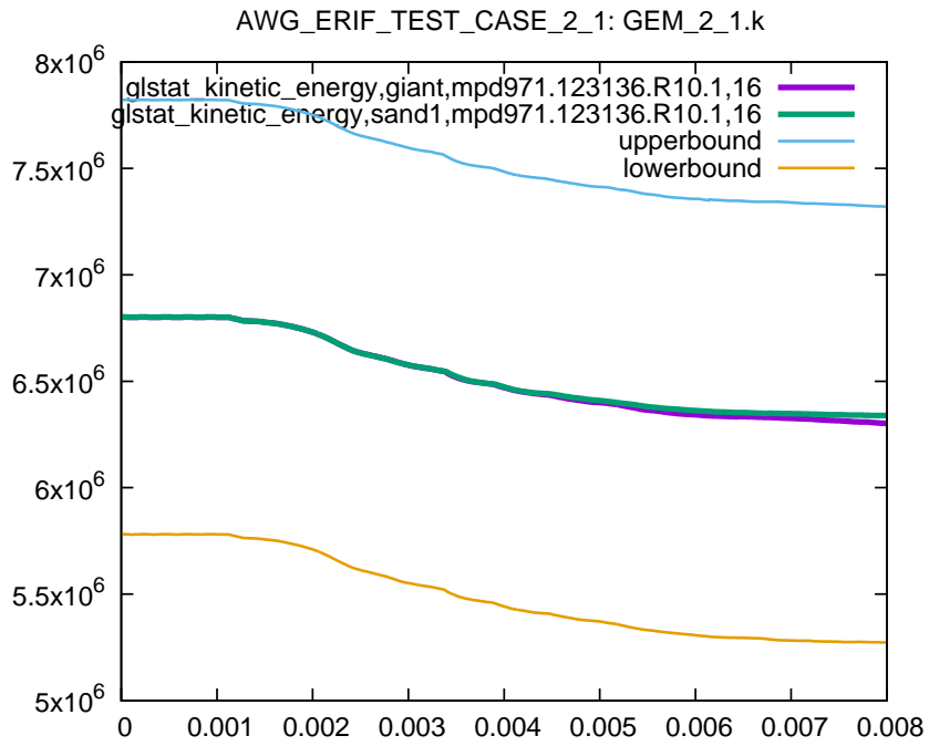
Figure 3: Global kinetic energy, sub test case ID 1
