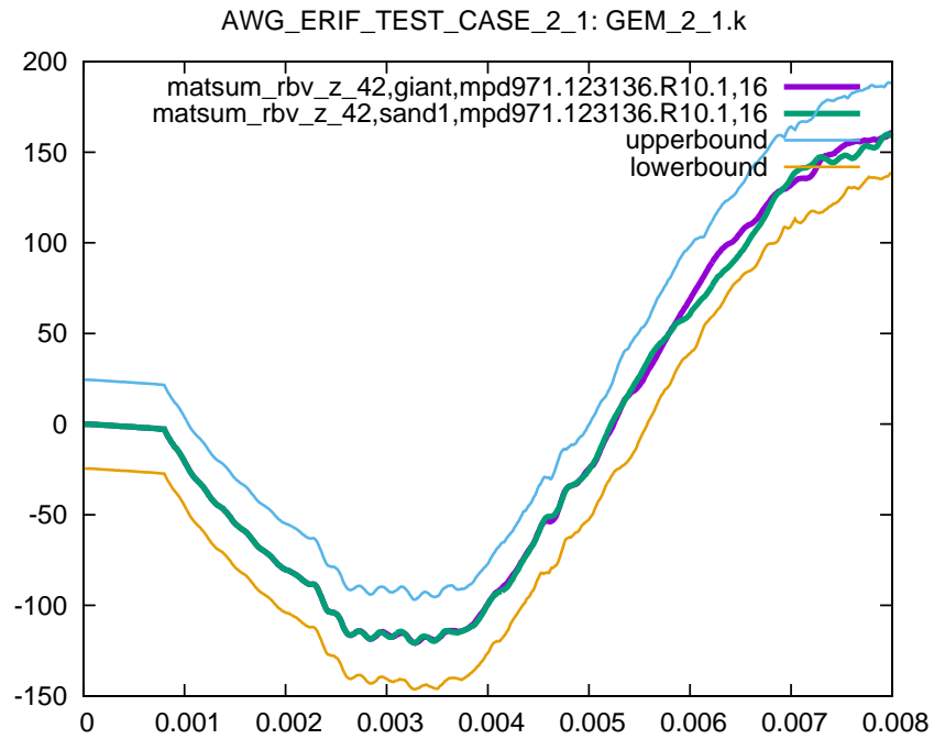
Figure 8: Rigid body velocity (z-component) part 42 (released blade), sub test case ID 1
