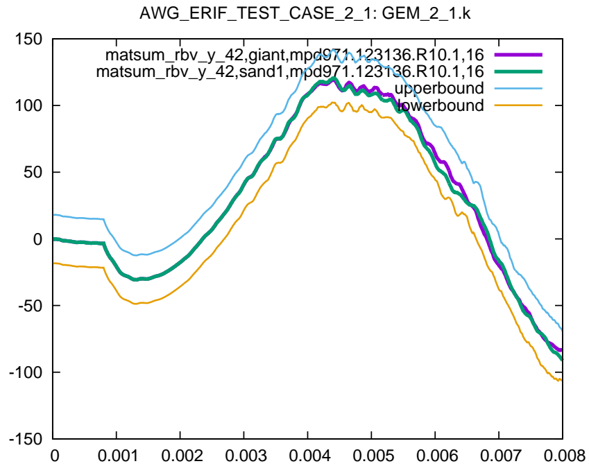
Figure 7: Rigid body velocity (y-component) part 42 (released blade), sub test case ID 1
