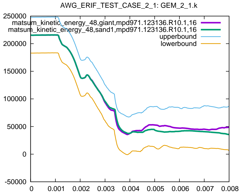
Figure 5: Kinetic energy part 48 (released blade), sub test case ID 1
