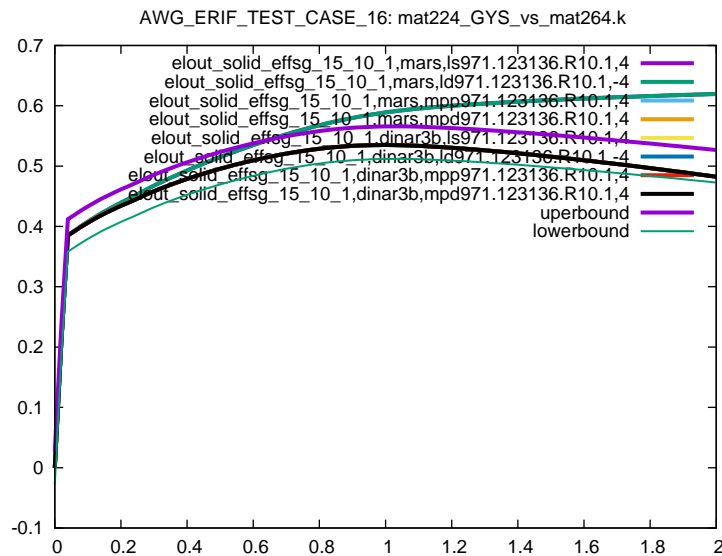
Figure 21: Cross platform results, Von Mises Stress, element ID 10, sub test case ID 1
