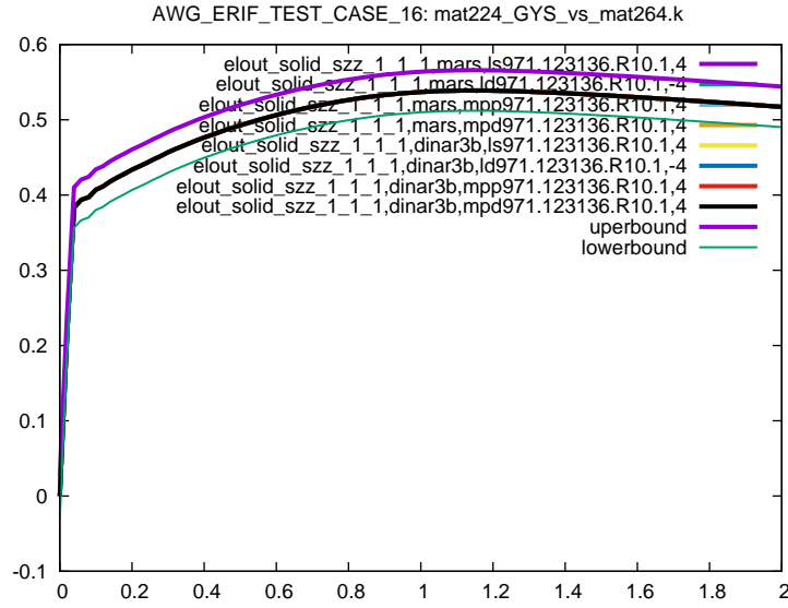
Figure 2: Cross platform results, z-component Stress, element ID 1, sub test case ID 1
