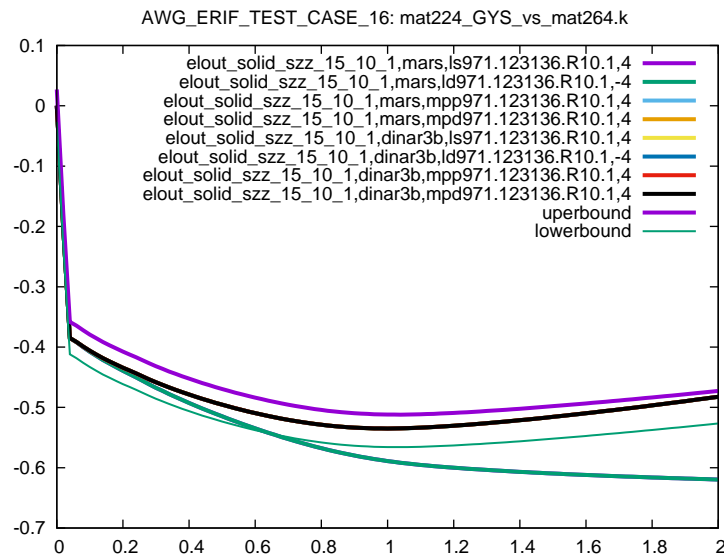
Figure 11: Cross platform results, z-component Stress, element ID 10, sub test case ID 1
