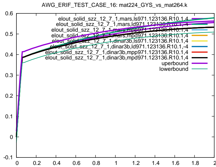
Figure 8: Cross platform results, z-component Stress, element ID 12, sub test case ID 1
