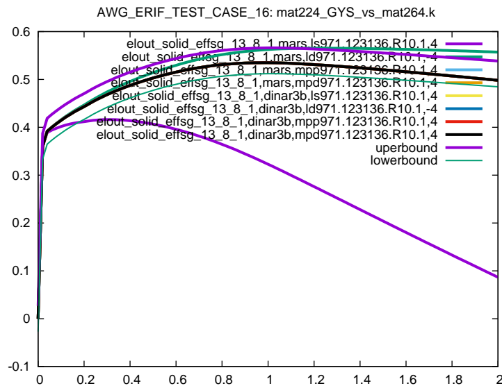
Figure 19: Cross platform results, Von Mises Stress, element ID 13, sub test case ID 1
