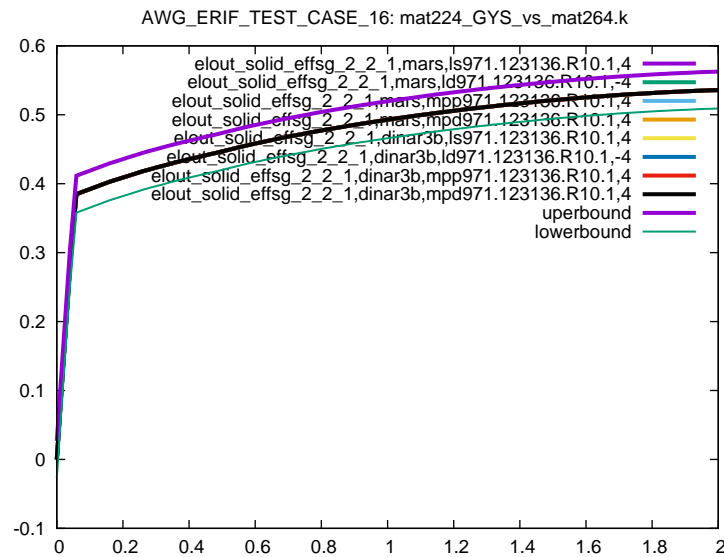
Figure 13: Cross platform results, Von Mises Stress, element ID 2, sub test case ID 1
