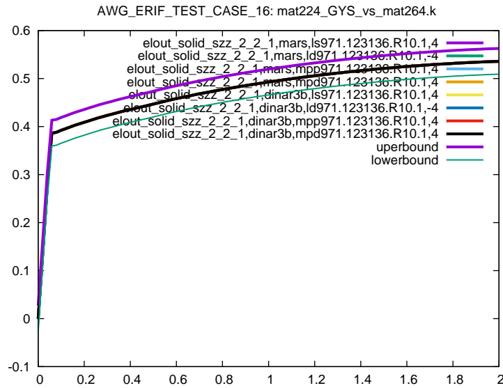
Figure 3: Cross platform results, z-component Stress, element ID 2, sub test case ID 1
