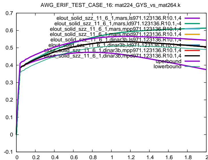
Figure 7: Cross platform results, z-component Stress, element ID 11, sub test case ID 1
