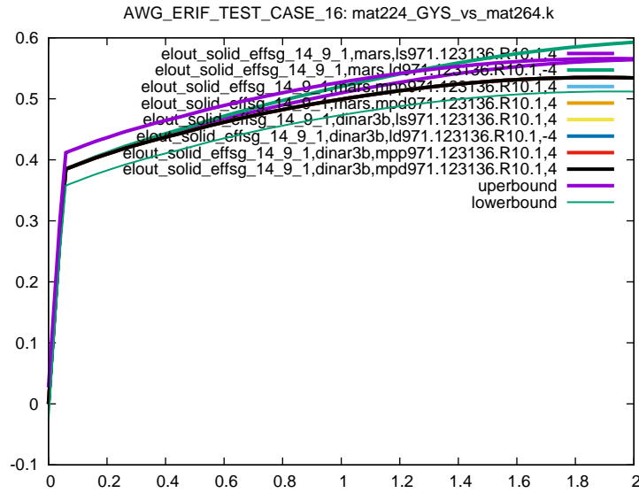
Figure 20: Cross platform results, Von Mises Stress, element ID 14, sub test case ID 1
