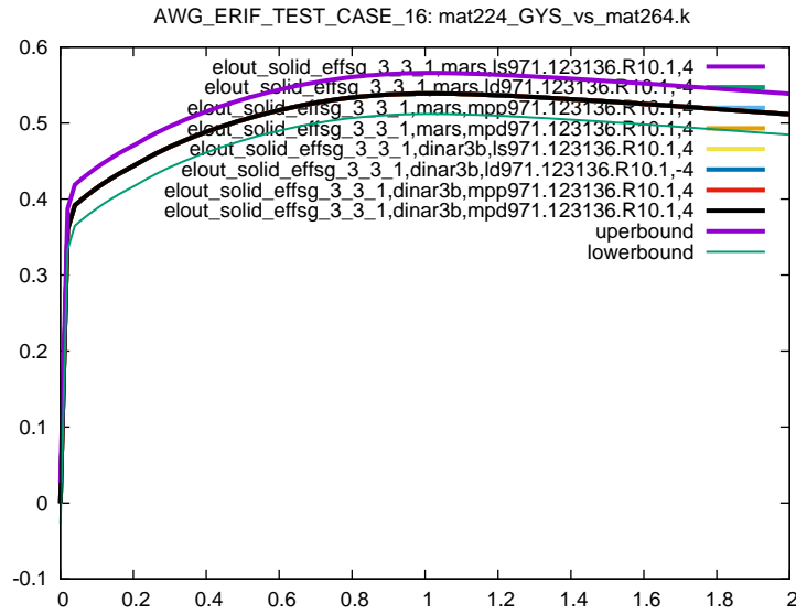
Figure 14: Cross platform results, Von Mises Stress, element ID 3, sub test case ID 1
