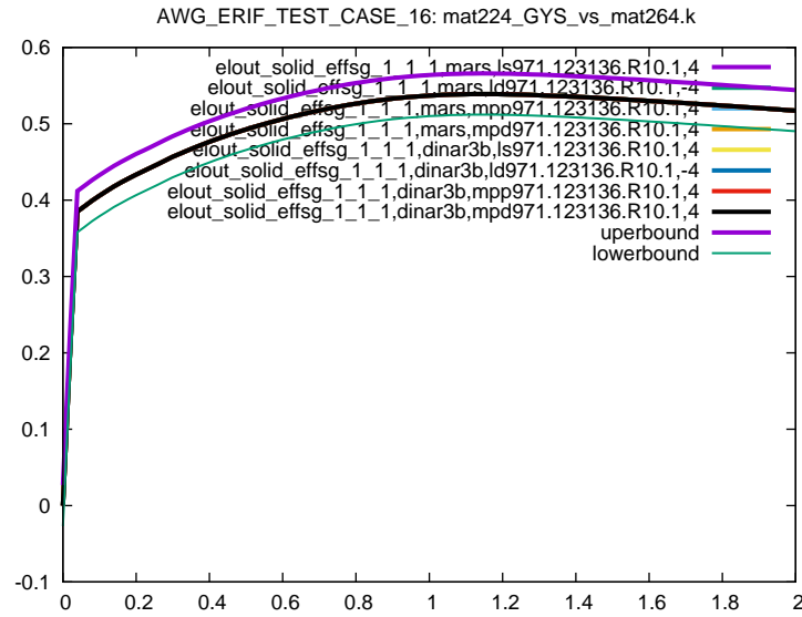
Figure 12: Cross platform results, Von Mises Stress, element ID 1, sub test case ID 1
