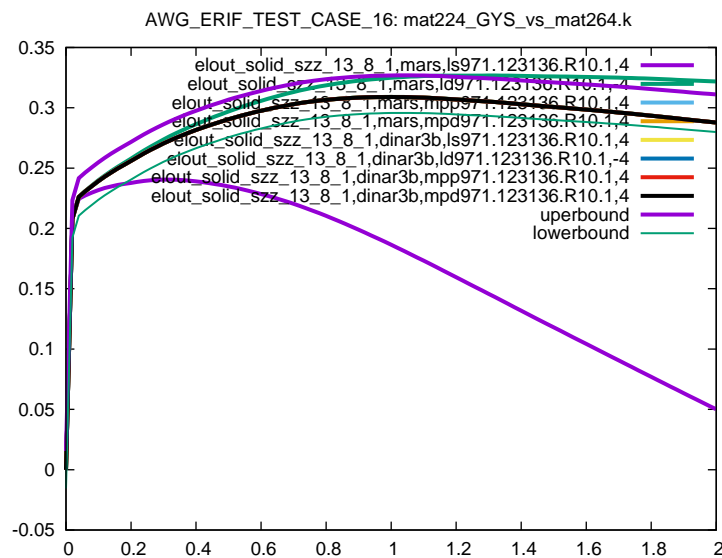
Figure 9: Cross platform results, z-component Stress, element ID 13, sub test case ID 1
