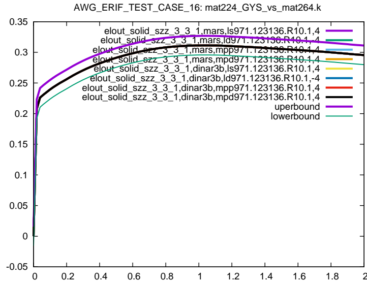
Figure 4: Cross platform results, z-component Stress, element ID 3, sub test case ID 1
