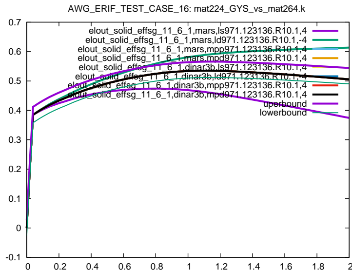
Figure 17: Cross platform results, Von Mises Stress, element ID 11, sub test case ID 1
