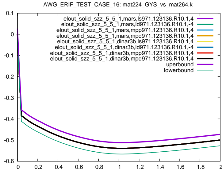
Figure 6: Cross platform results, z-component Stress, element ID 5, sub test case ID 1
