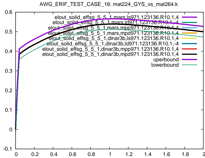
Figure 16: Cross platform results, Von Mises Stress, element ID 5, sub test case ID 1
