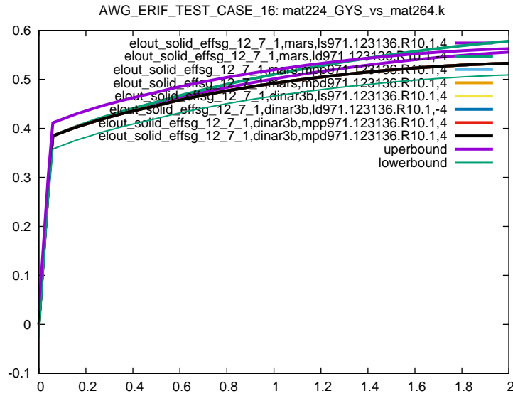
Figure 18: Cross platform results, Von Mises Stress, element ID 12, sub test case ID 1
