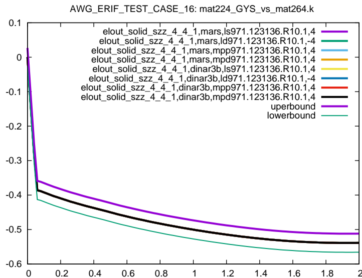
Figure 5: Cross platform results, z-component Stress, element ID 4, sub test case ID 1
