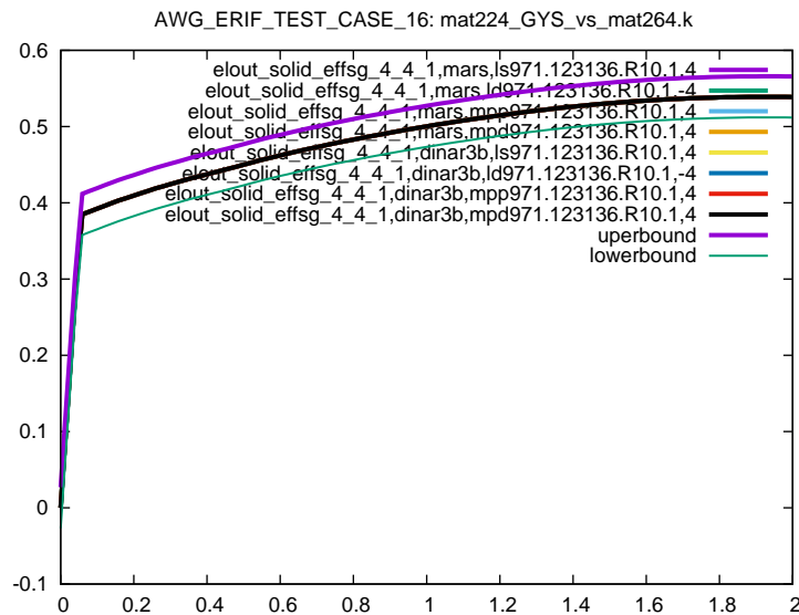
Figure 15: Cross platform results, Von Mises Stress, element ID 4, sub test case ID 1
