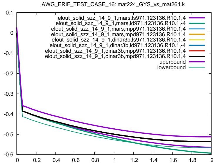
Figure 10: Cross platform results, z-component Stress, element ID 14, sub test case ID 1
